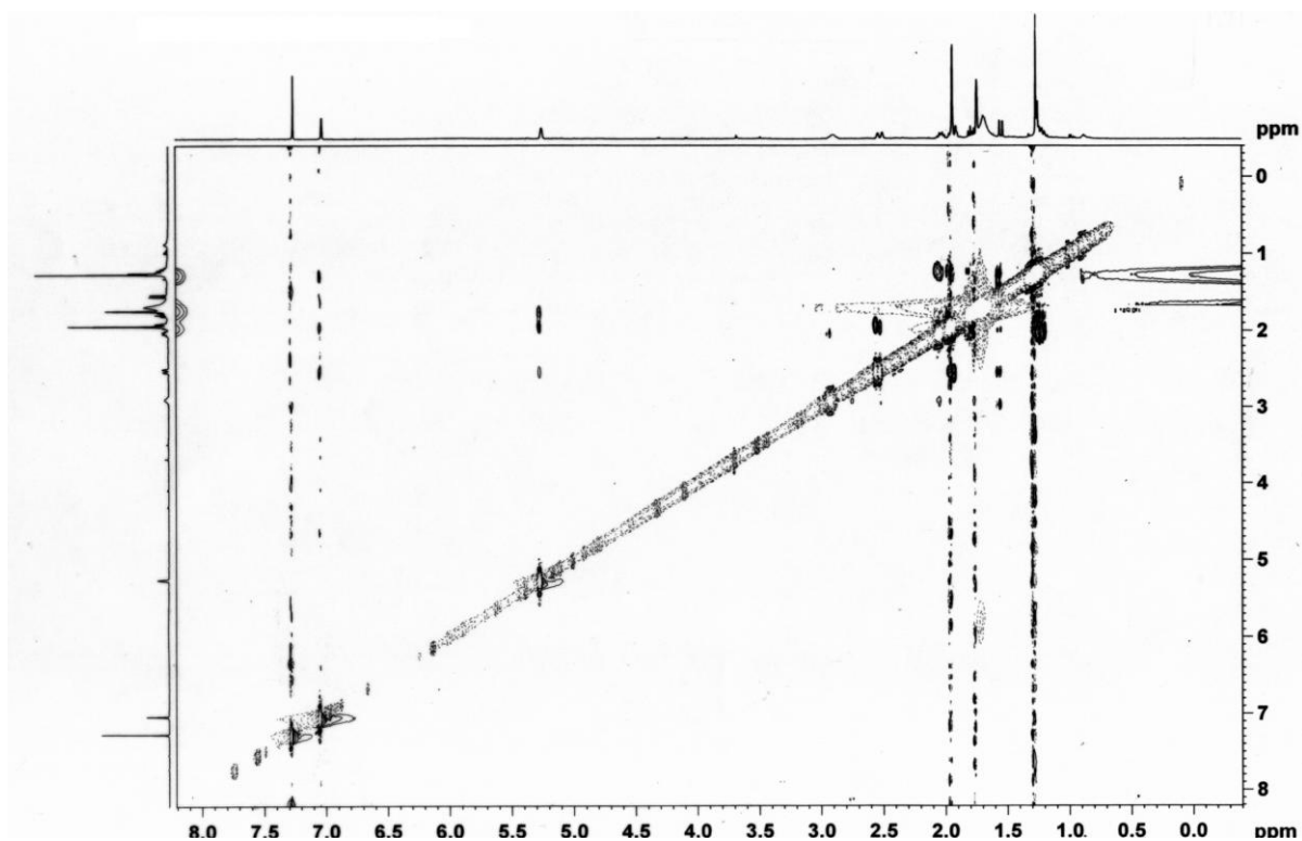
Figure S10. NOESY Spectrum of sinularianin D (4) in \text{CDCl}_3 (500 MHz).
