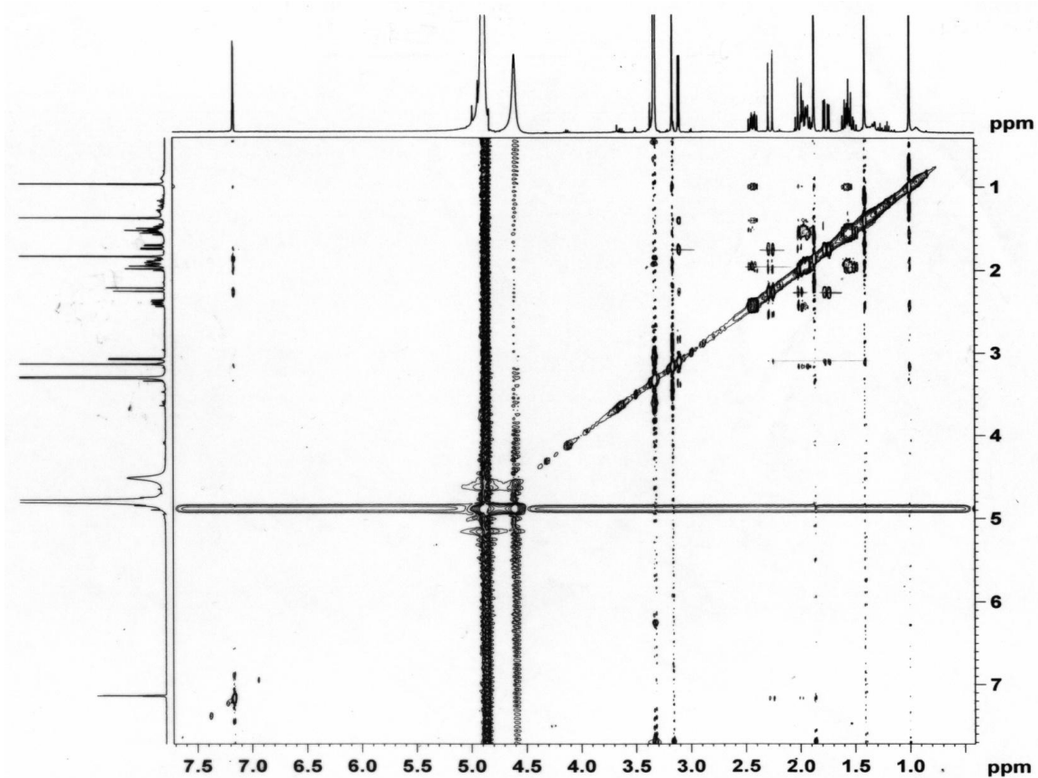
Figure S6. NOESY Spectrum of sinularianin C ( 3 ) in CD 3 OD (500 MHz).
