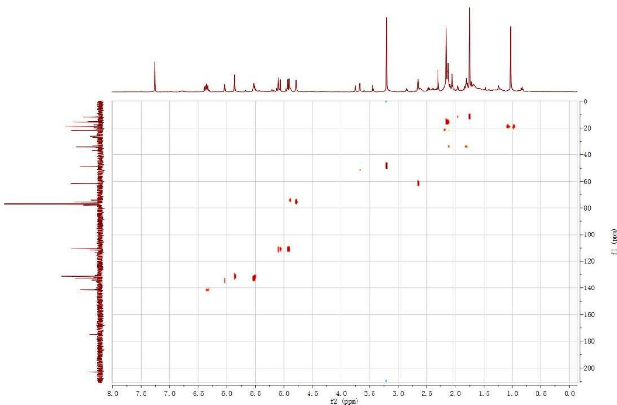
Figure S20. HMBC Spectrum of sinularianin F (6) in CDCl 3 (500 MHz).
