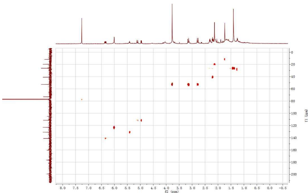
Figure S14. HMQC Spectrum of sinularianin E (5) in \text{CDCl}_3 (500 MHz).
