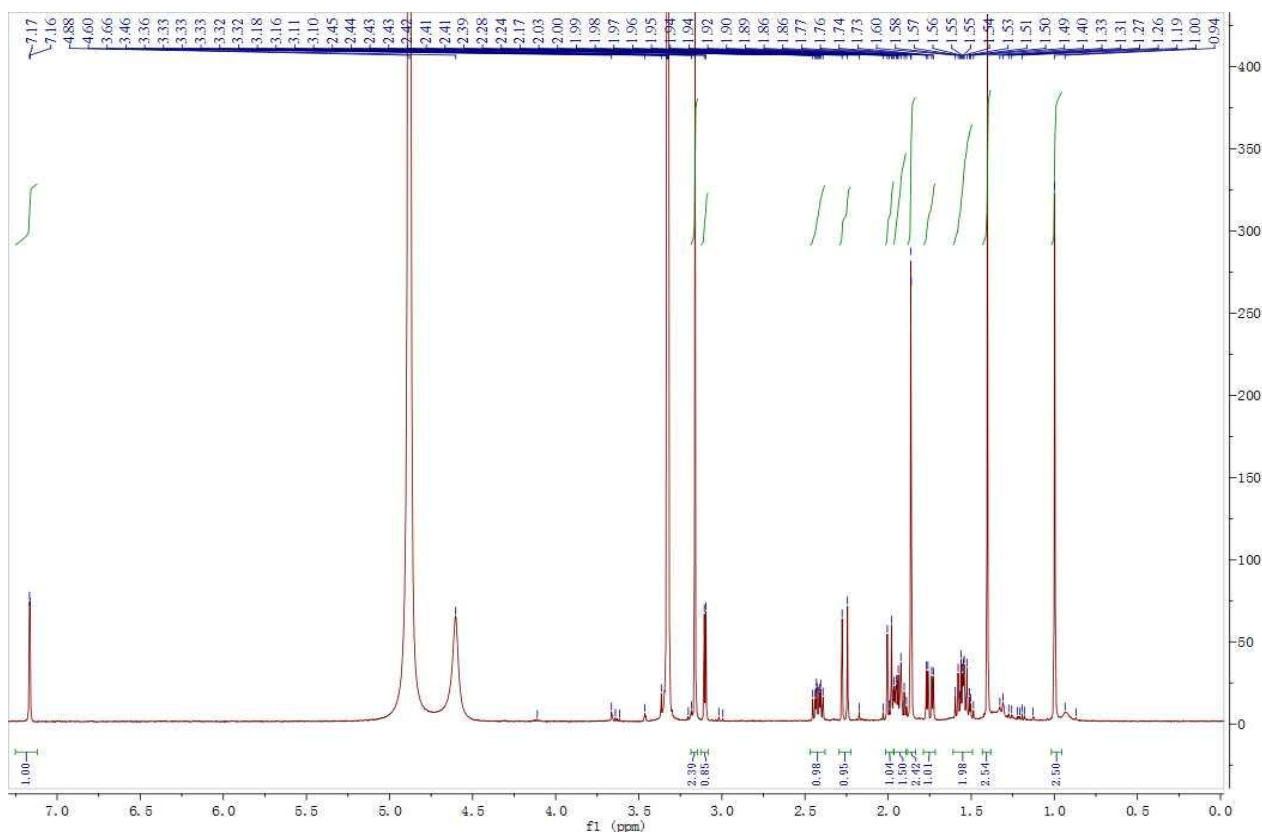
Figure S2. 1 H NMR Spectrum of sinularianin C (3) in CD 3 OD (500 MHz).
