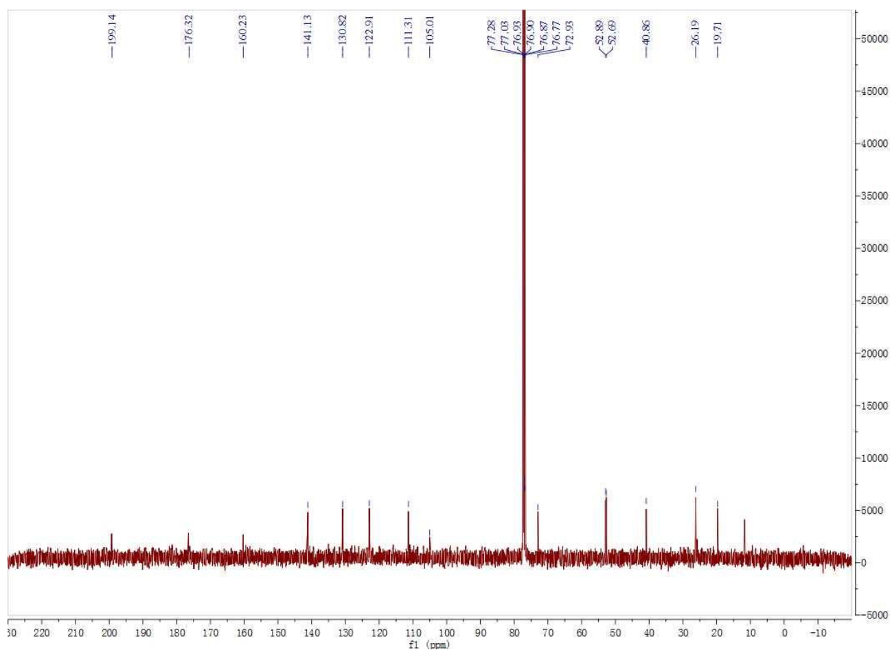
Figure S14. HMQC Spectrum of sinularianin E (5) in \text{CDCl}_3 (500 MHz).
