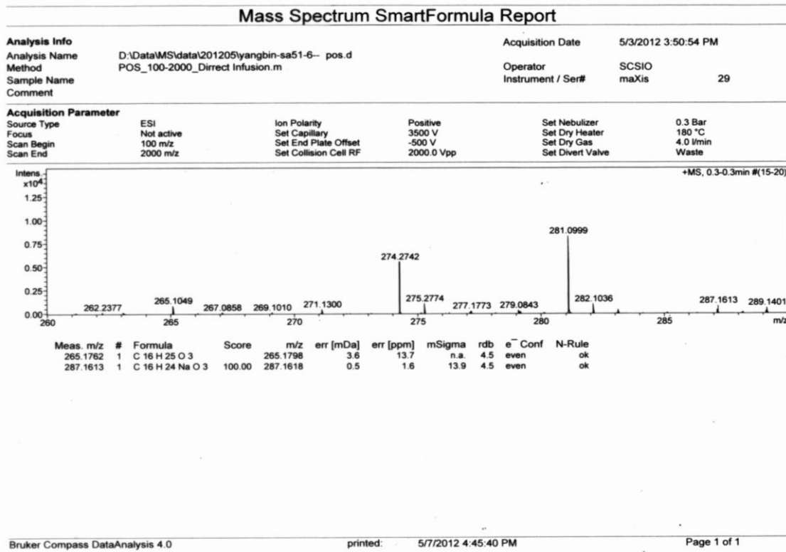
Figure S16. HR-ESI-MS Spectrum of sinularianin F (6).
