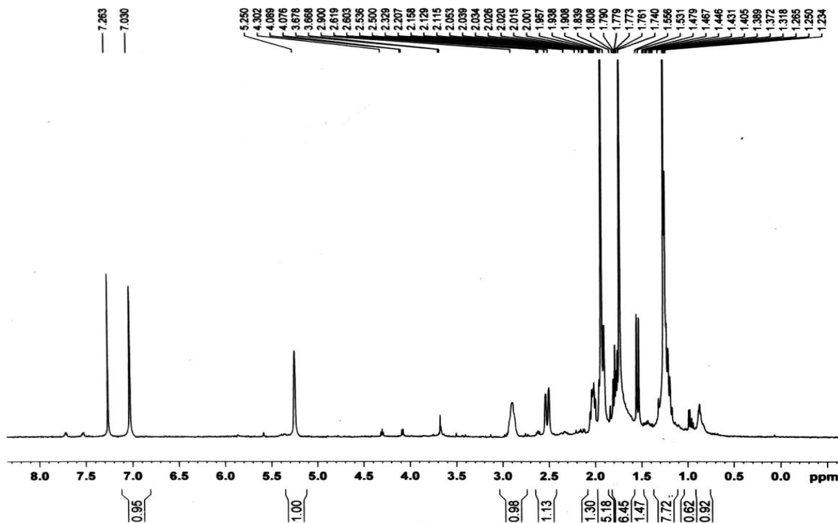
Figure S8. 1 H NMR Spectrum of sinularianin D (4) in CDCl 3 (500 MHz).
