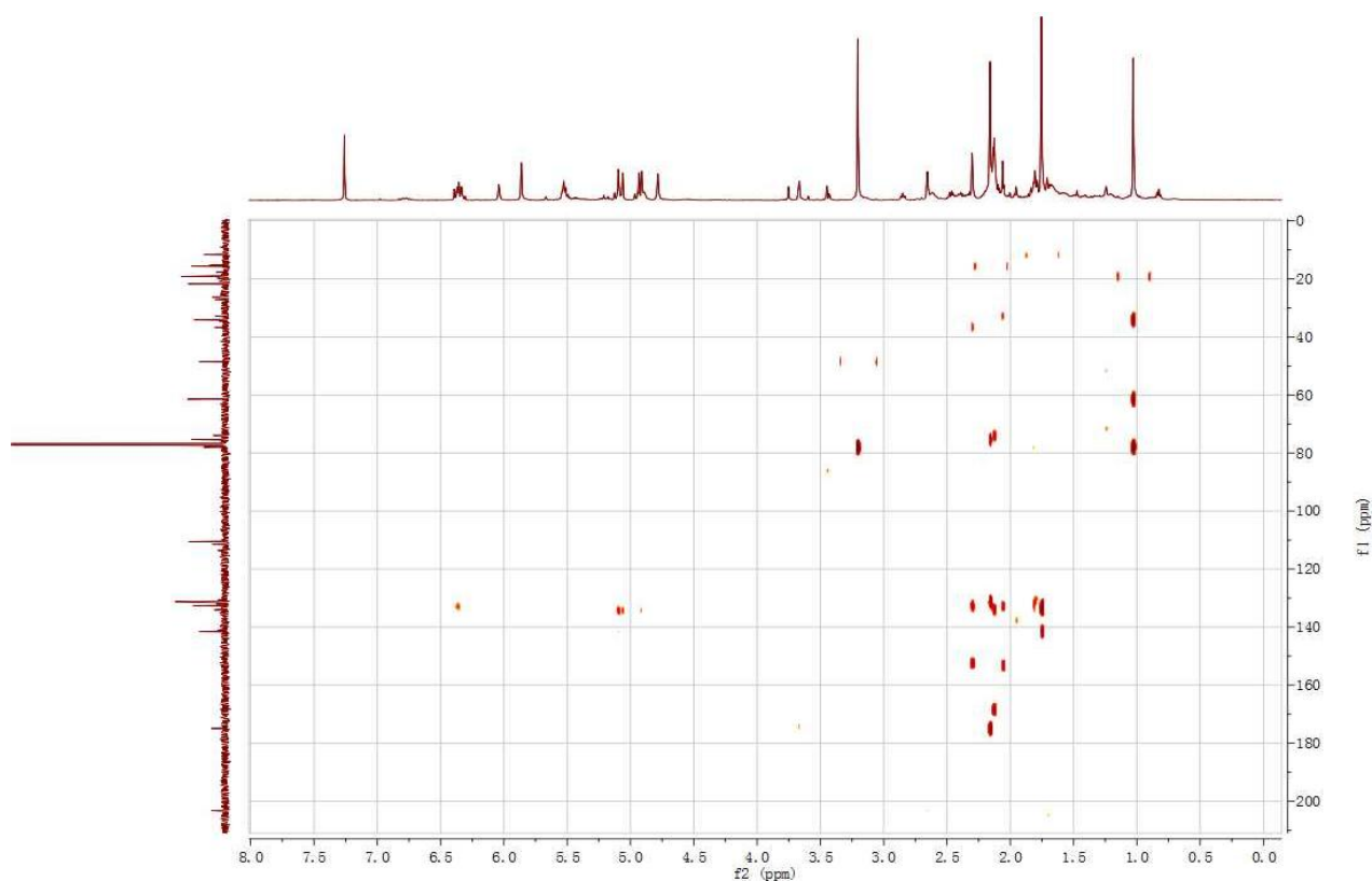
Figure S20. HMBC Spectrum of sinularianin F (6) in CDCl 3 (500 MHz).
