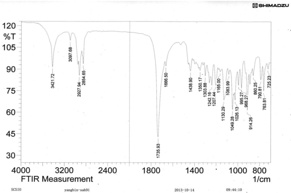
Figure S21. IR Spectra of sinularianin D (4).
