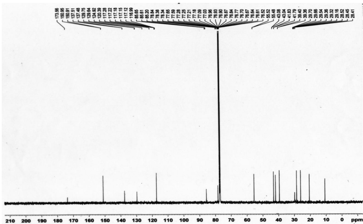
Figure S10. NOESY Spectrum of sinularianin D (4) in \text{CDCl}_3 (500 MHz).
