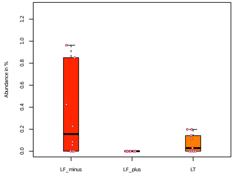
Arcobacter
