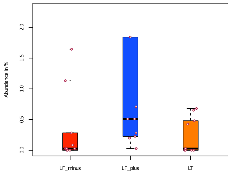
Schlegellella
