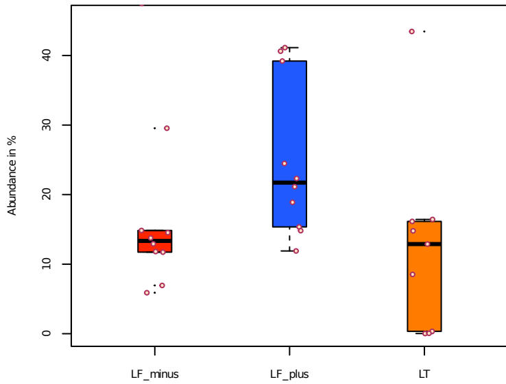
Acinetobacter
