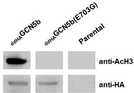
Figure S1. In vitro HAT assays using recombinant histone H3 and either purified _{ddHA} GCN5b or _{ddHA} GCN5b(E703G). Proteins were purified from parasites cultured in the presence of 500 nM Shield for 48 hours. KAT reactions were analyzed by Western blotting with antibody recognizing acetylated H3. Parental strain was used as a negative control. Anti-HA was used to show that the same approximate amount of protein was used in each assay.
