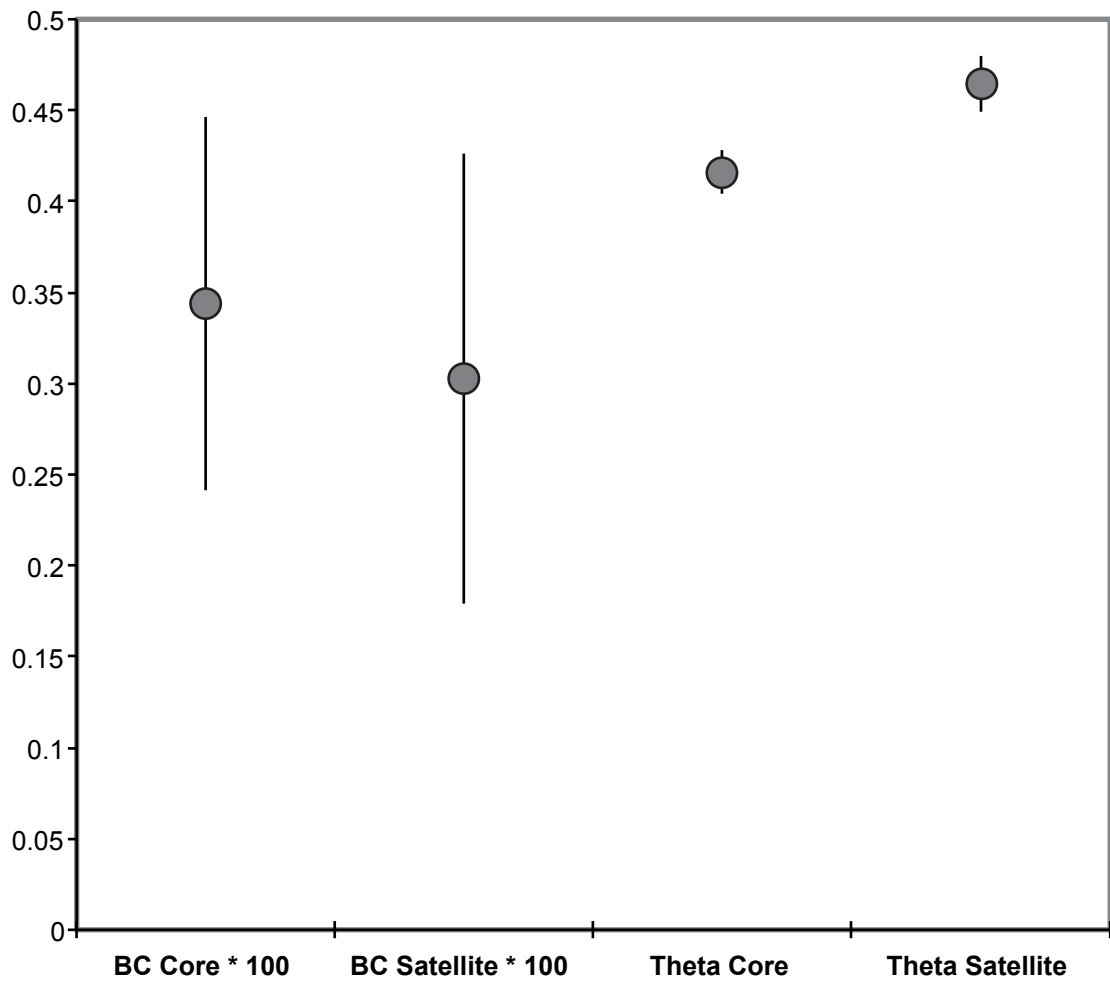
Figure S2. Comparison of 74 genes with capsid and replication-associated functions, compared to the 75 other genes, grouped as 'core' or 'satellite' respectively (Zanotto & Krakauer, 2008). The median values of betweenness centrality (BC) and genetic diversity ( \theta ) and the associated standard errors are shown. BC values were multiplied by 100 for comparative scaling with \theta .
