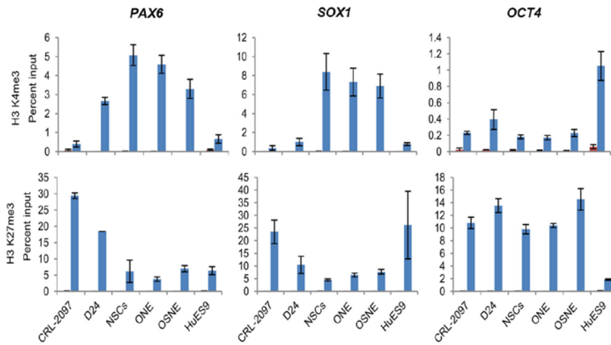
Supplementary information, Figure S8 Histone modification during direct reprogramming. PAX6 , SOX1 , and OCT4 promoter loci were analyzed by chromatin immunoprecipitation with anti-H3K4me3 and H3K27me3 antibodies. hNSCs derived from HuES9, reprogrammed hiNSCs (ONE and OSNE) and HuES9 were used as controls. Blue bars represent the extent of immunoprecipitation from anti-modified histone antibodies and red bars from normal IgG.
