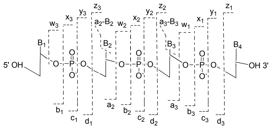
Oligonucleotide Fragmentation Nomenclature
