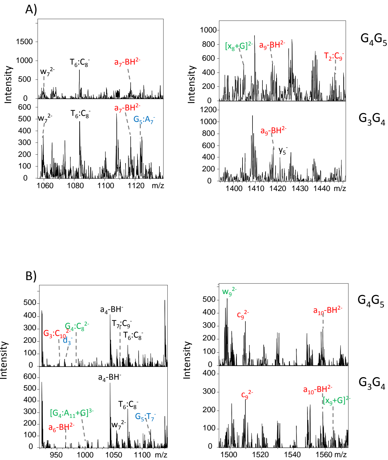
Supplemental Figure 2. Expanded regions of IRMPD spectra for (A) G3-D/cisplatin and (B) G3-H/cisplatin adducts showing some of the diagnostic fragment ions that allow differentiation of the adducts.
