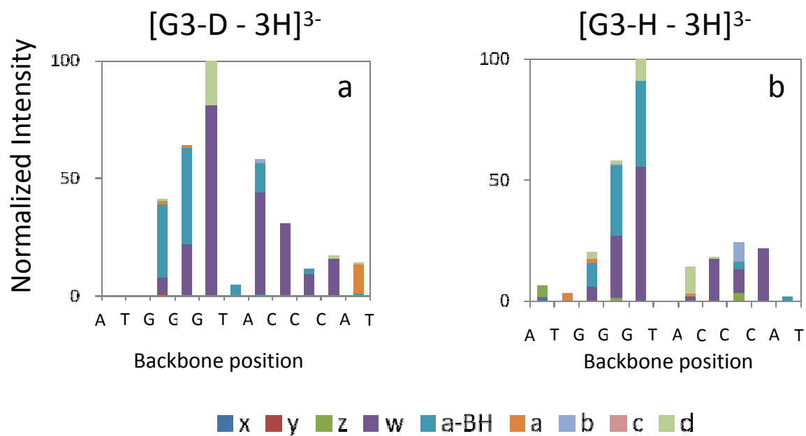
Supplemental Information Figure 3. Relative abundances of IRMPD fragment ions at each backbone cleavage site for (a) all fragments of [G3-D-3H] 3- ; (b) all fragments of [G3-H-3H] 3- .
