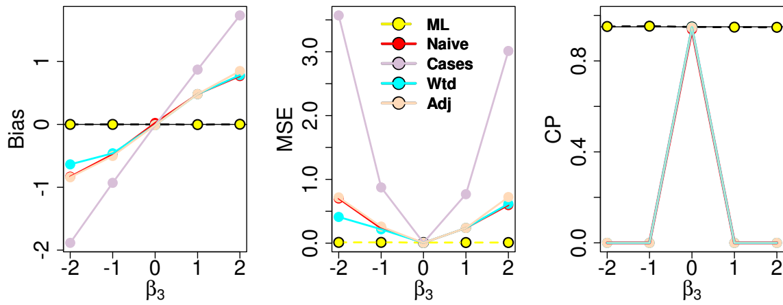
Figure 4: Performances of the naïve, cases-only (“Cases”), weighted (“Wtd”), and the adjusted (“Adj”) estimators compared to the ML estimator for binary secondary trait
