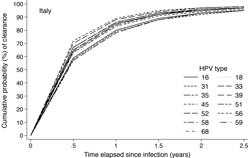
Figure S2.1. Estimated median cumulative probability (%) of HPV infection clearance, by HPV type and country.
