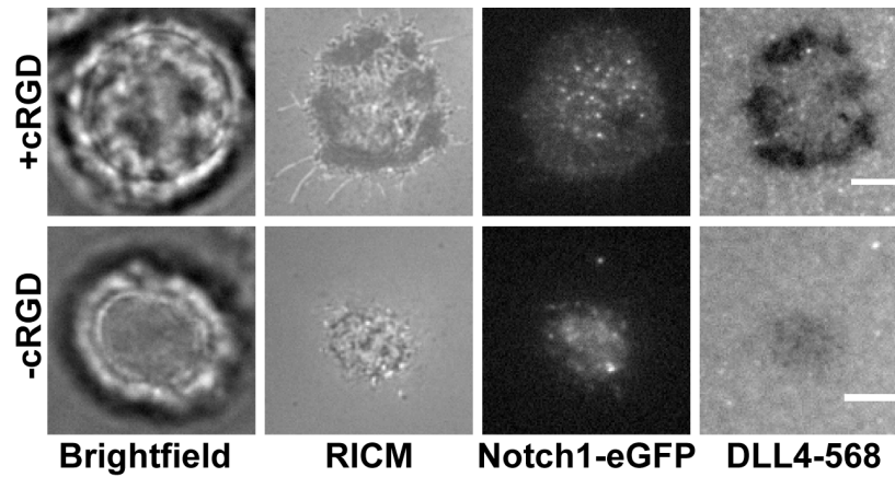
Figure S3. Specificity of DLL4 binding to Notch1. Notch1-eGFP cells were treated with soluble DLL4/Fc (185 nM) for 20 min before incubating on a DLL4-568 membrane surface. In order to facilitate imaging of cells, cRGD was added to the supported lipid membrane (top) to promote cell adhesion. Without cRGD-integrin binding, the Notch1-eGFP expressing cells very weakly associated with the supported lipid membrane (bottom).
