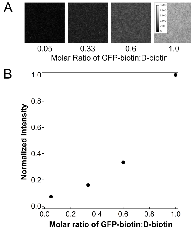
Figure S13. Competitive binding experiment between GFP-biotin and D-biotin on a lipid membrane. In this experiment, GFP-biotin was selected as a model ligand in place of DLL4-mCherry-biotin. The goal was to titrate different molar ratios of biotinylated (fluorescent) ligand to D-biotin on a membrane surface and to observe the effect on fluorescence intensity. First, eGFP \alpha -thioester (expressed and purified using the IMPACT kit from New England Biolabs, Ipswich, MA) was site specifically modified with cysteine-biotin (Carbosynth, San Diego, CA) using expressed protein ligation (3). The resulting GFP-biotin was incubated on a streptavidin functionalized 0.1 mol% biotin-DPPE membrane at a series of molar ratios of GFP-biotin to D-biotin. The total biotin concentration was maintained at 250 nM. (A) Representative epifluorescence images of biotin-DPPE membranes incubated with different molar ratios of GFP-biotin to D-biotin. (B) Plot illustrating the fluorescence intensity as a function of the molar ratio of GFP-biotin to D-biotin. This plot was used to make an initial estimate for the amount of free D-biotin needed to produce a 4 mol% biotin-DPPE bilayer with the same ligand density (fluorescence intensity) as a 0.1 mol% biotin-DPPE surface.
