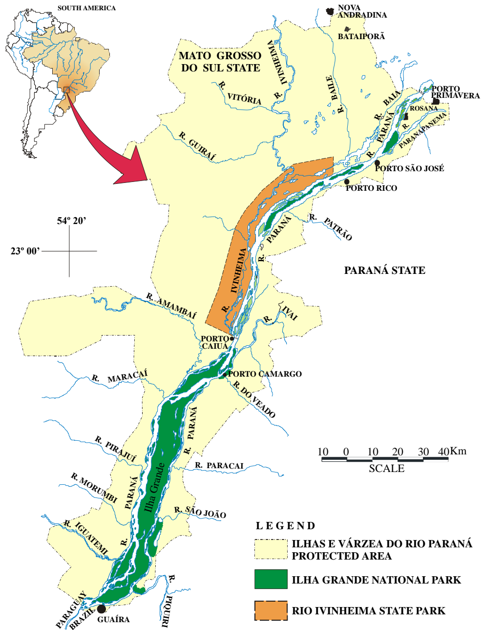
Figure S1. Location of the Upper Paraná River and its floodplain, associated environmental protection areas, and extent of the LTER site. The floodplain extends up to 20 km from the western margin of the Paraná River, primarily in the area of influence of the Ivinheima and Baía rivers.
