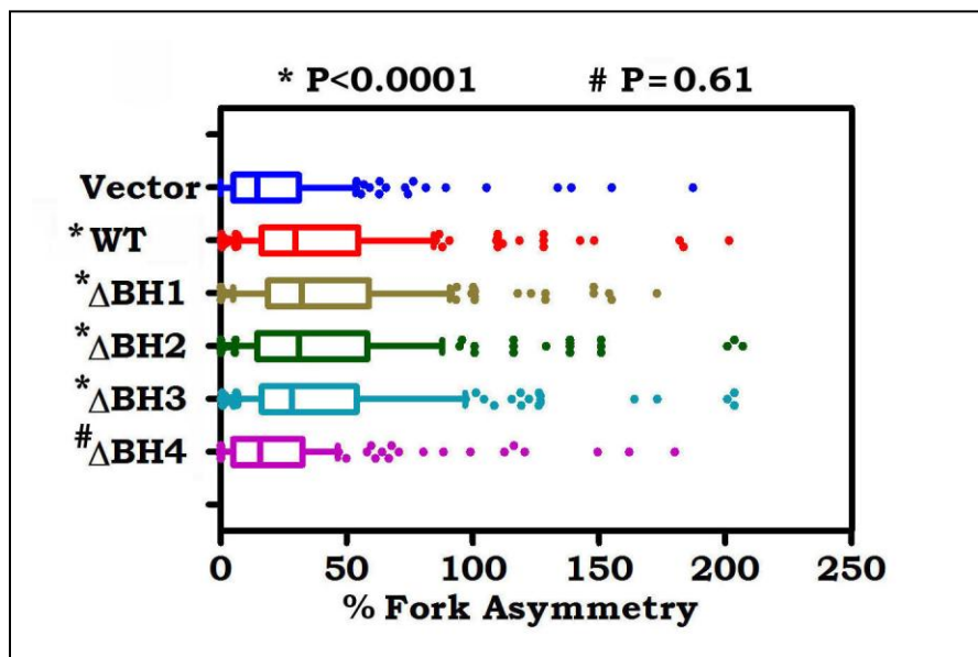
Figure S5. The BH4 domain is essential for Bcl2 to cause the asymmetrical DNA replication. Distribution of the degree of asymmetry of bidirectional replication forks was compared in H1299 cells expressing WT or each of BH deletion Bcl2 mutants.
