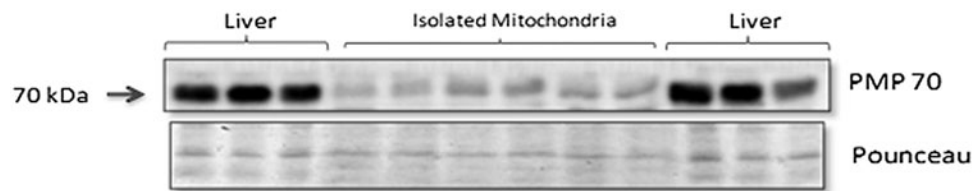
SUPPLEMENTARY FIG. S1. Expression of PMP 70 in mitochondrial suspension. Liver homogenates were used as positive controls.
