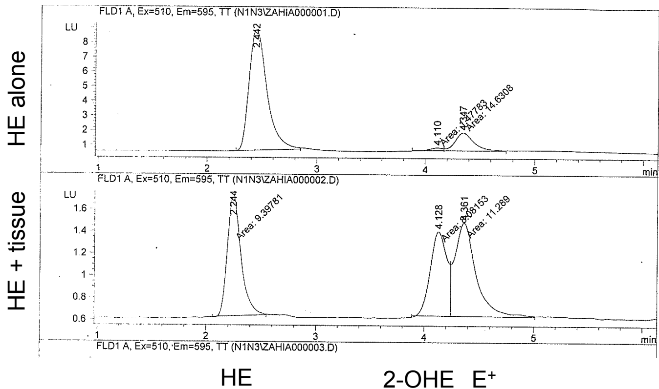
Supplemental Figure I. Representative HPLC readouts illustrating measurement of HE oxidation after exposure to aortic tissue (bottom) versus HE alone (top). HE = hydroethidine, 2-OHE = 2-hydroxyethidium, E + = ethidium.
