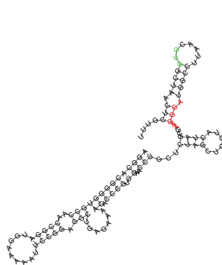
predicted ydaO-yuaA leader - RF 000379 5'-UTR of cg2402
