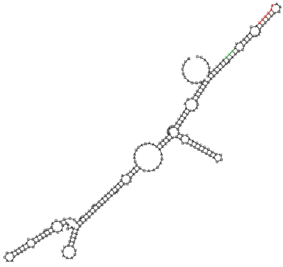
predicted FMN riboswitch - RF 00050 5'-UTR of cg0083
