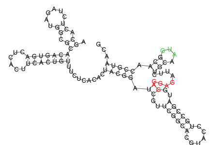
predicted yybP-ykoY leader - RF 00080 5'-UTR of cg2157/terC
