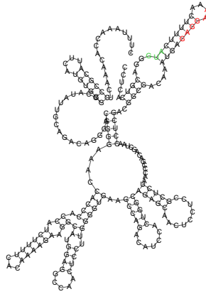
predicted ydaO-yuaA leader - RF 000379 5'-UTR of cg0936/rpf1
