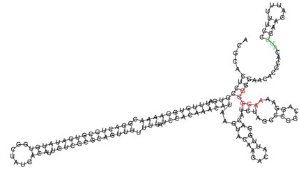
predicted mraW RNA motif - RF 01746 5'-UTR of cg2377/mraW
