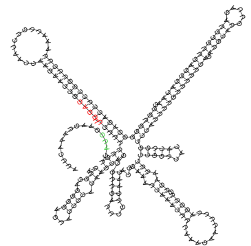
predicted yybP-ykoY leader - RF 00080 5'-UTR of cg2157/terC
