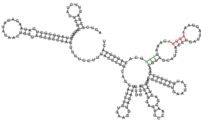
predicted TPP riboswitch - RF 00059 5'-UTR of cg0825
