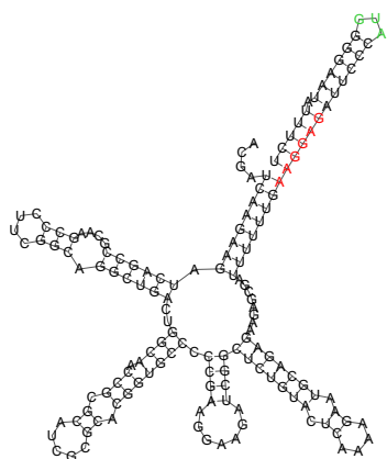
predicted SAM-IV riboswitch - RF 000634 5'-UTR of cg1478
