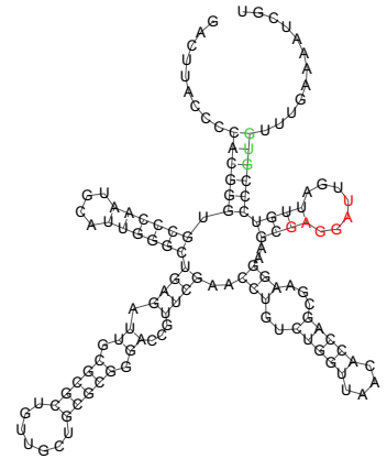
predicted TPP riboswitch - RF 00059 5'-UTR of cg2236/thiE
