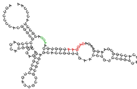
predicted TPP riboswitch - RF 00059 5'-UTR of cg1476/thiC
