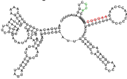
predicted TPP riboswitch - RF 00059 5'-UTR of cg0825
