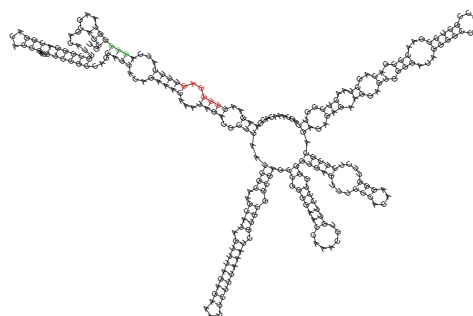
predicted ydaO-yuaA leader - RF 000379 5'-UTR of cg2402
