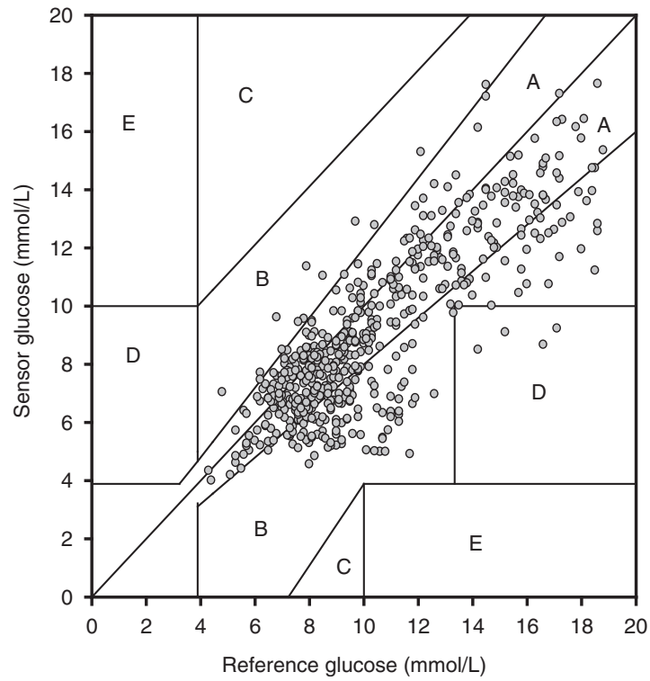
SUPPLEMENTARY FIG. S1. Clarke error grid using (top panel) the enhanced calibration protocol and (bottom panel) the standard calibration protocol (manufacturer's instructions).
