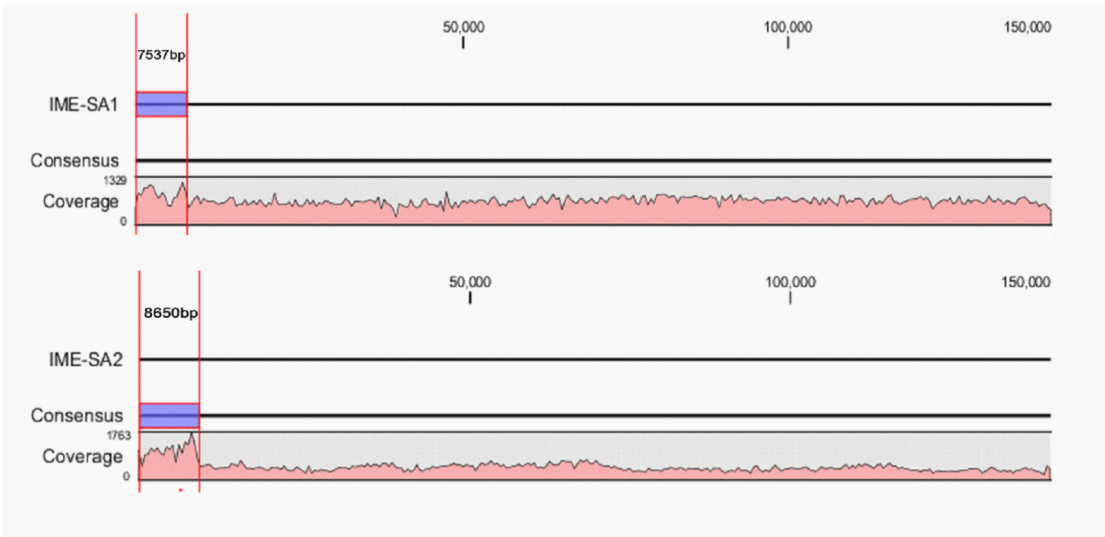
Figure S3. The mapping of S. aureus phage IME-SA1 and IME-SA2. S. aureus phage genome has about 8000bp long terminal repeats at the ends of their genome.
