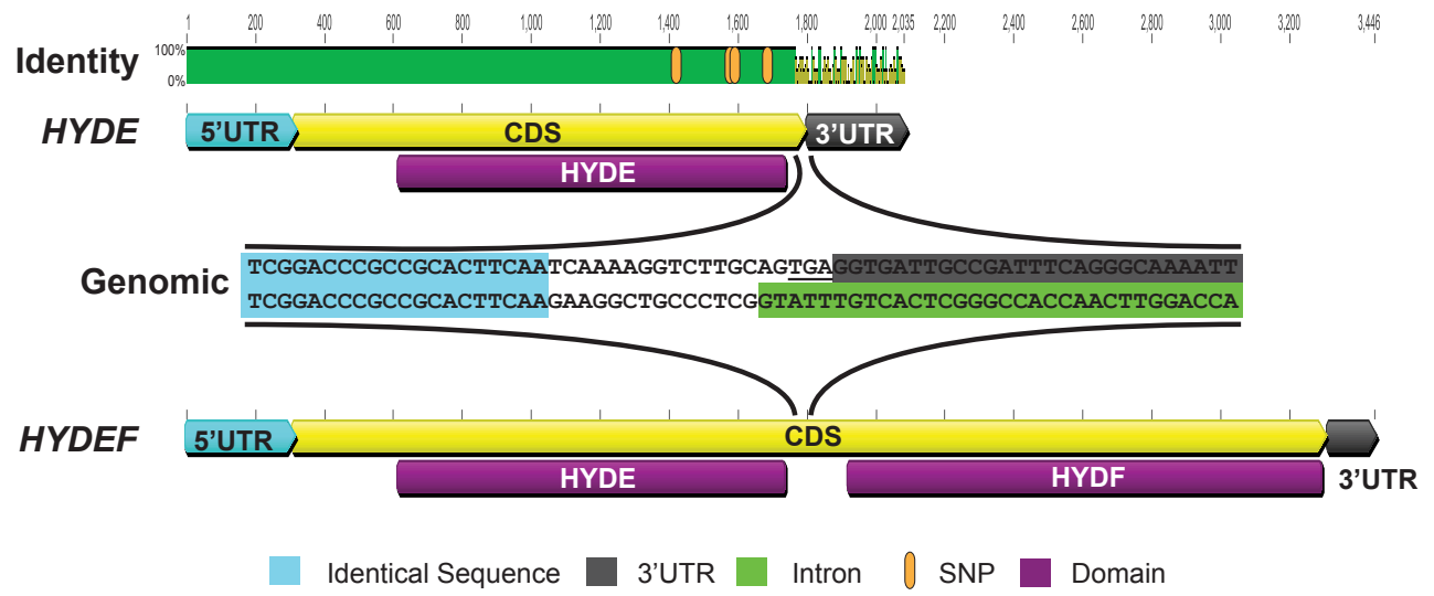
Figure S1. Schematic representation of the independent HYDE and fused HYDEF transcripts obtained from transcriptome sequencing.
