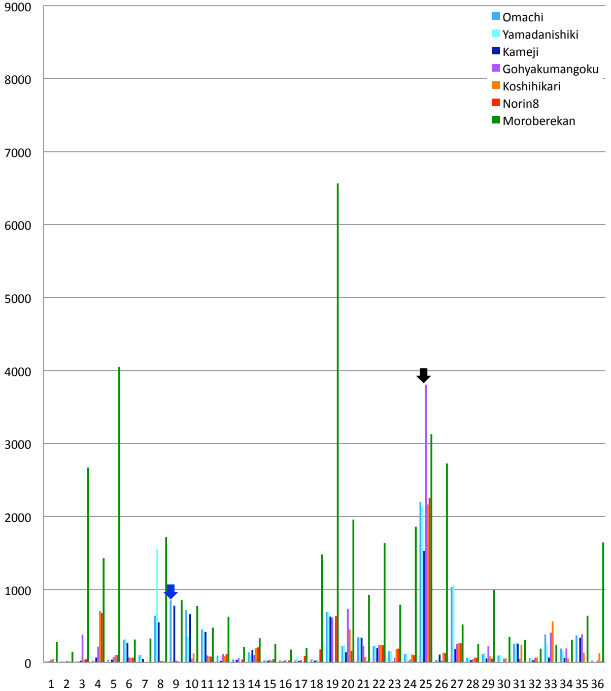
Figure S3. Distribution of SNPs between the different cultivars and Nipponbare reference sequence across the chromosome 2. The x-axis represents the physical distance along each chromosome, split into 1 Mb windows. The y-axis indicates the number of SNPs. The black arrows show the high-density regions common among the 7 cultivars. The blue arrows show the remarkably different regions between Omachi and Yamadanishiki.
