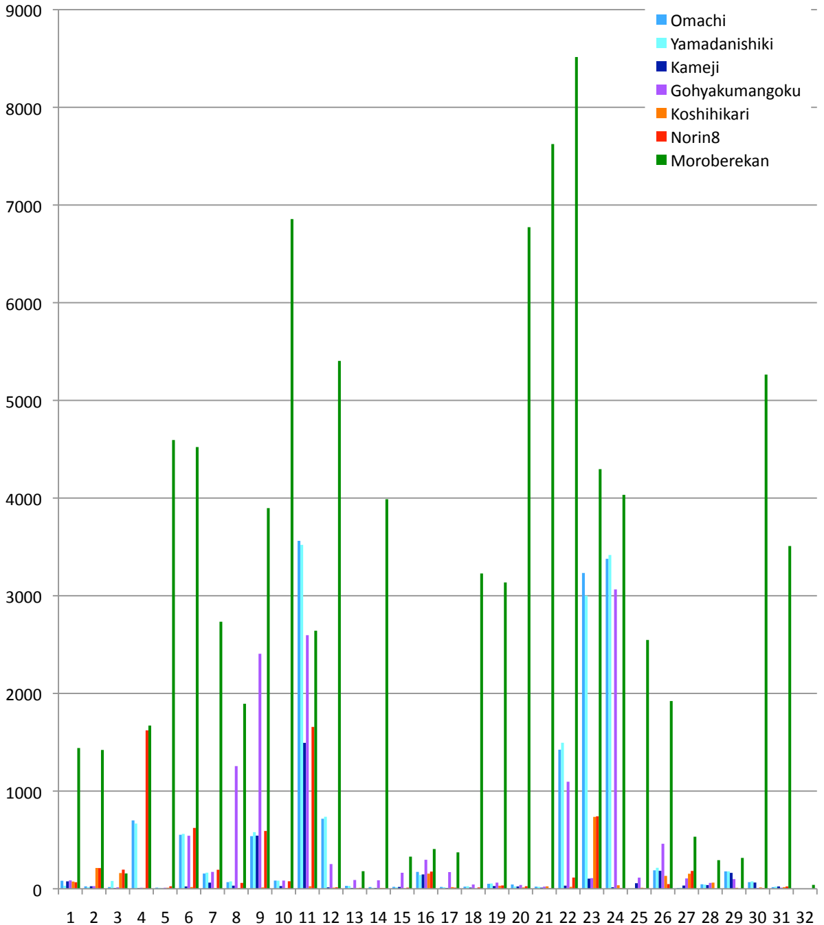
Figure S7. Distribution of SNPs between the different cultivars and Nipponbare reference sequence across the chromosome 6. The x-axis represents the physical distance along each chromosome, split into 1 Mb windows. The y-axis indicates the number of SNPs.
