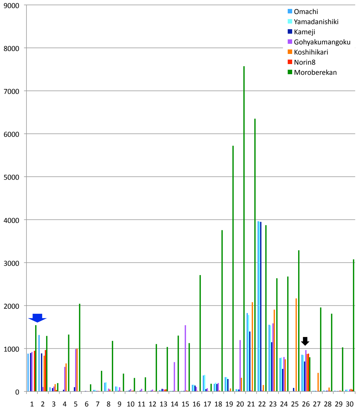
Figure S8. Distribution of SNPs between the different cultivars and Nipponbare reference sequence across the chromosome 7. The x-axis represents the physical distance along each chromosome, split into 1 Mb windows. The y-axis indicates the number of SNPs. The black arrows show the high-density regions common among the 7 cultivars. The blue arrows show the remarkably different regions between Omachi and Yamadanishiki.
