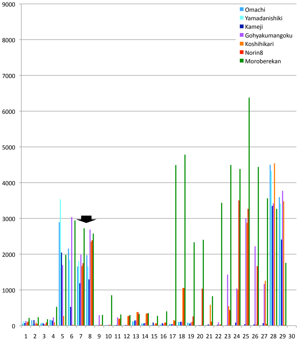
Figure S12. Distribution of SNPs between the different cultivars and Nipponbare reference sequence across the chromosome 11. The x-axis represents the physical distance along each chromosome, split into 1 Mb windows. The y-axis indicates the number of SNPs. The black arrows show the high-density regions common among the 7 cultivars.
