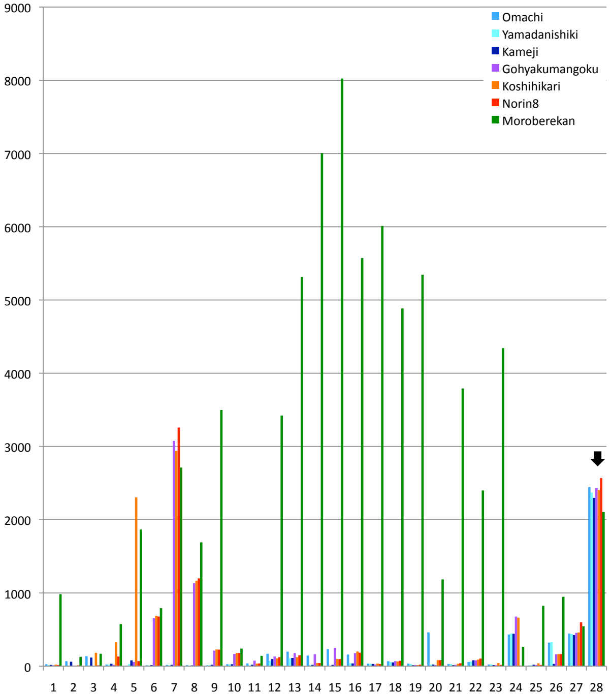
Figure S13. Distribution of SNPs between the different cultivars and Nipponbare reference sequence across the chromosome 12. The x-axis represents the physical distance along each chromosome, split into 1 Mb windows. The y-axis indicates the number of SNPs. The black arrows show the high-density regions common among the 7 cultivars.
