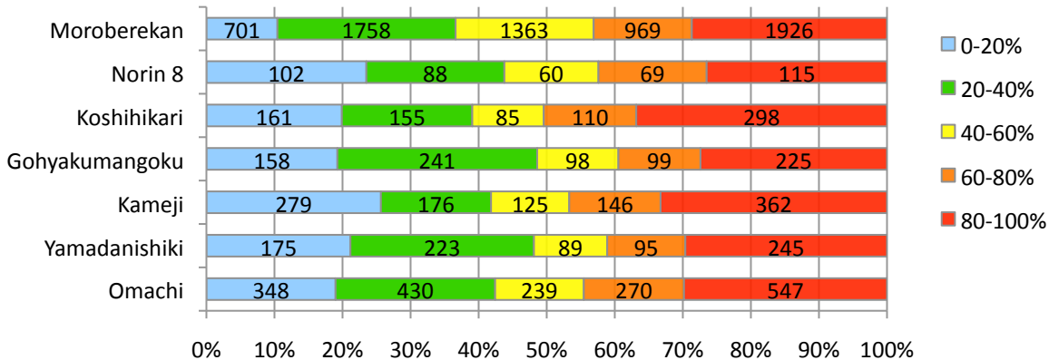
Figure S14. The degree of unique hit sequences in the contig sequences. The results are shown by colour boxes classified to 5 groups on the basis of percentages of the alignment length in the contig length: 0–20% (blue), 20–40% (green), 40–60% (yellow), 60–80% (orange), and 80–100% (red). The numbers in the bars show the number of contigs.
