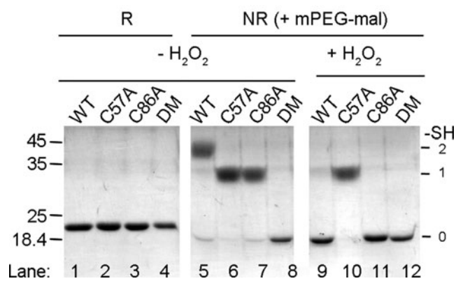
SUPPLEMENTARY FIG. S4. Cys57 is responsible for H 2 O 2 reaction. The indicated GPx7 variants (20 \mu M) were incubated without ( lanes 1–8 ) or with 40 \mu M H 2 O 2 ( lanes 9–12 ). Samples were then treated by adding NR 2 \times SDS-loading buffer containing 10 mM mPEG-mal ( lanes 5–12 ) or reducing (R) SDS-loading buffer ( lanes 1–4 ), and resolved by SDS-15% PAGE. The numbers of thiols modified by mPEG-mal were indicated on the right margin.
