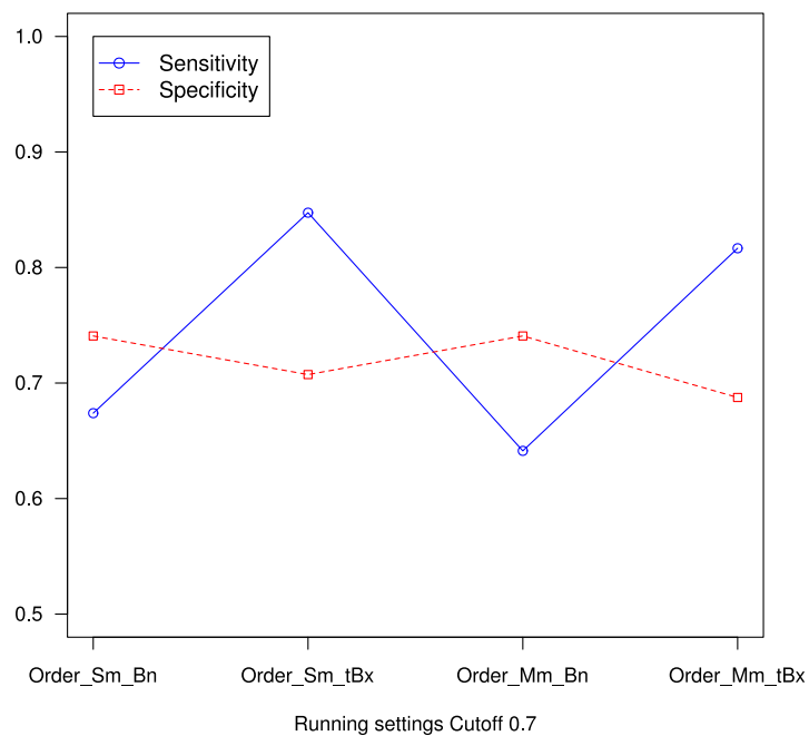
PhymmBL Sensitivity and Specificity at Order Level
