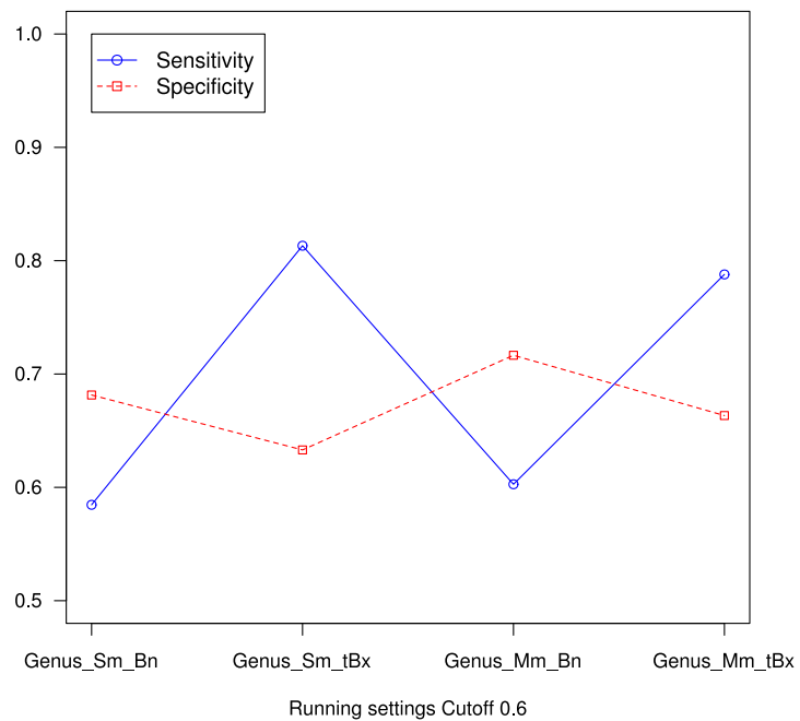
PhymmBL Sensitivity and Specificity at Genus Level
