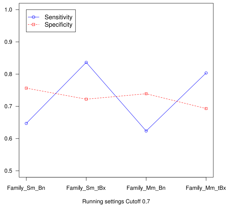
PhymmBL Sensitivity and Specificity at Family Level
