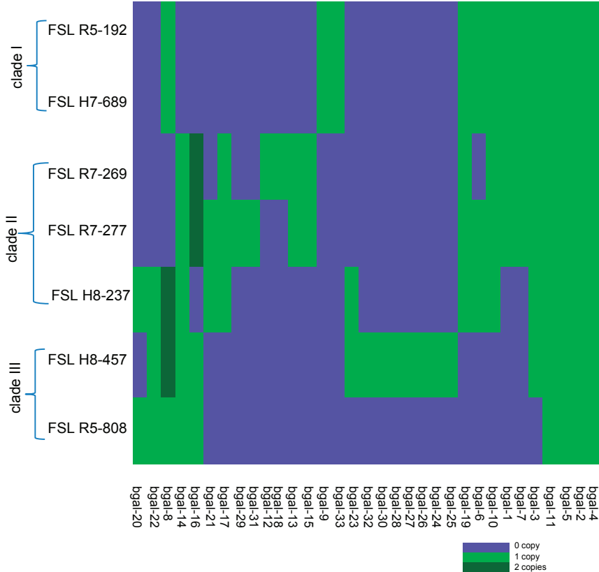
Additional file 8. Heatmap of the distribution of \beta -galactosidases in the seven Paenibacillus genomes. Blue indicates absence, green indicates presence, and dark green indicates two copies of a given \beta -galactosidase
