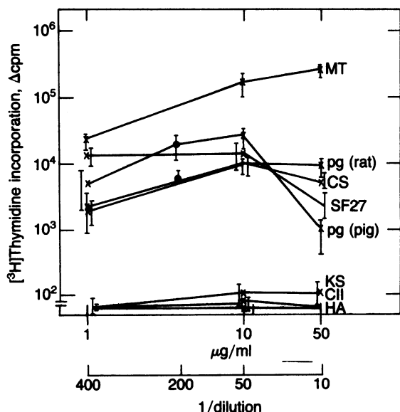
FIG. 1. In vitro ^3\text{H} )thymidine incorporation by the arthritogenic T-lymphocyte clone A2b after stimulation by M. tuberculosis (MT) and various cartilage components. pg, Proteoglycan preparation of rat or pig cartilage; CS, conditioned medium of chicken chondrocyte culture; SF27, cell-free synovial fluid from a human osteoarthritic knee.
