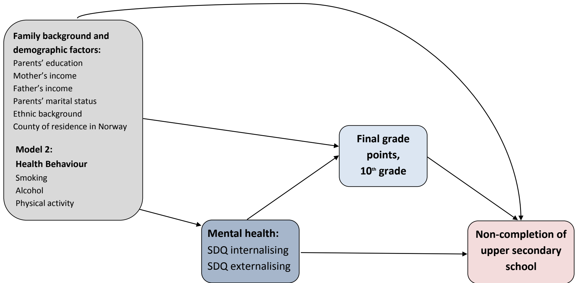
Additional file 1: Figure S1- The model assumed in the causal mediation analyses.
