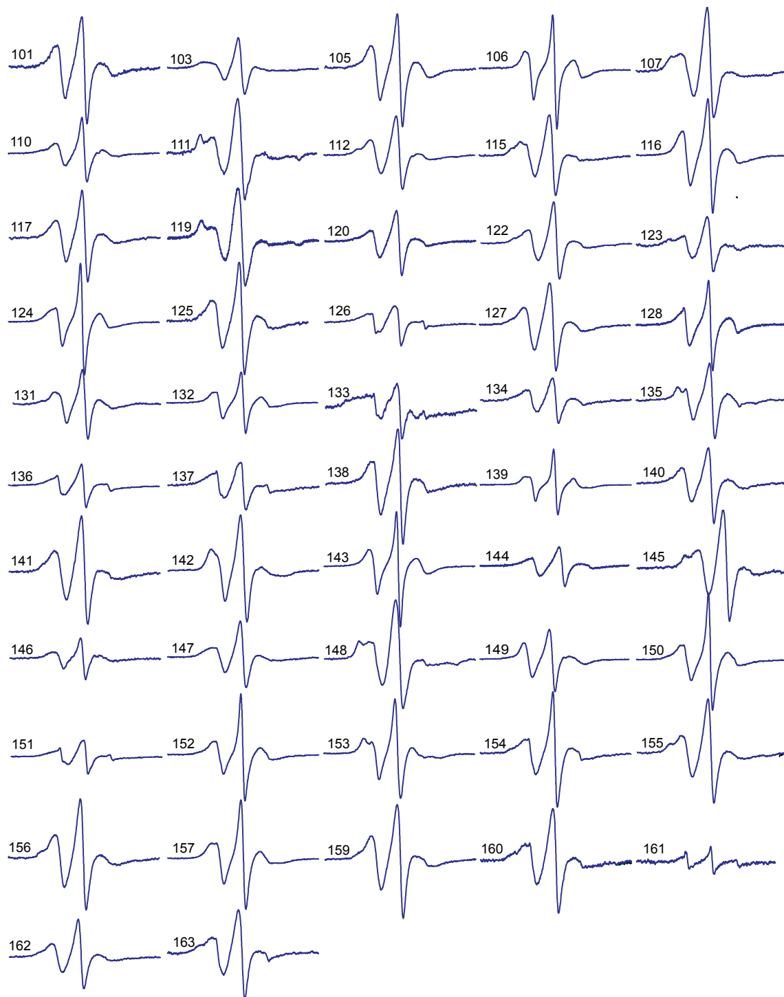
Fig S1. Examples of EPR spectra of spin-labeled apoA-I proteins within the 99-163 region of the primary sequence.
