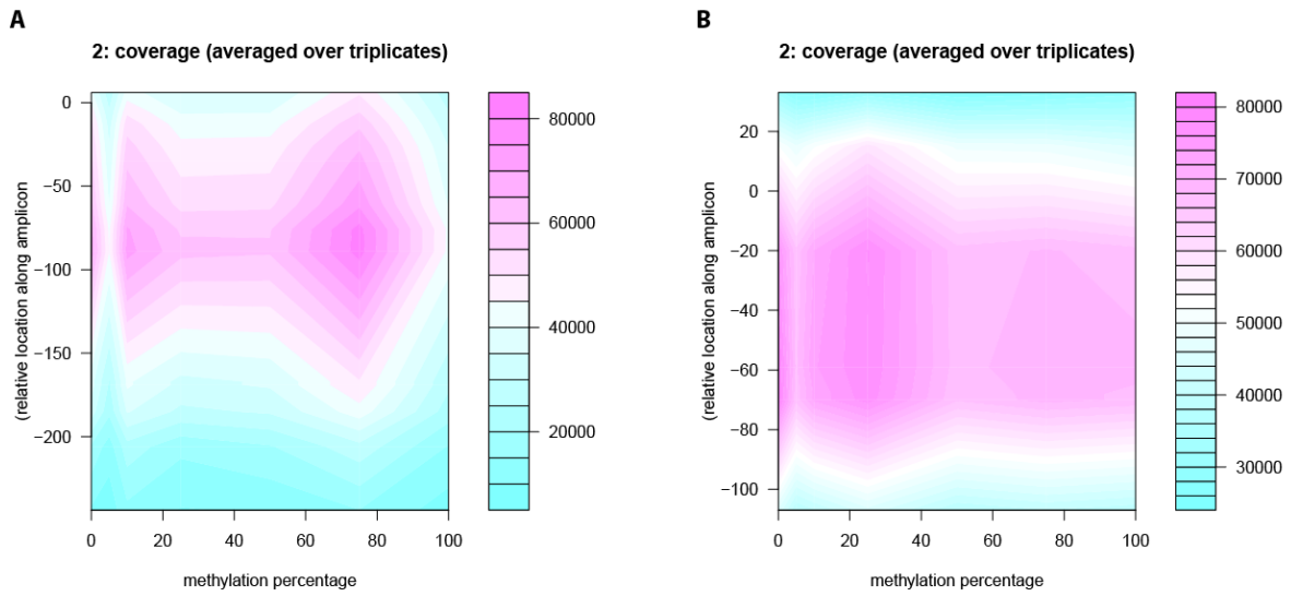
Supplemental Figure 2: Depth plots across mouse and rat amplicons for BSAS. A) Average sequencing depth plots across mouse amplicon and B) rat amplicon for each methylation standard. Relative location along amplicon in reference to transcription start site.
