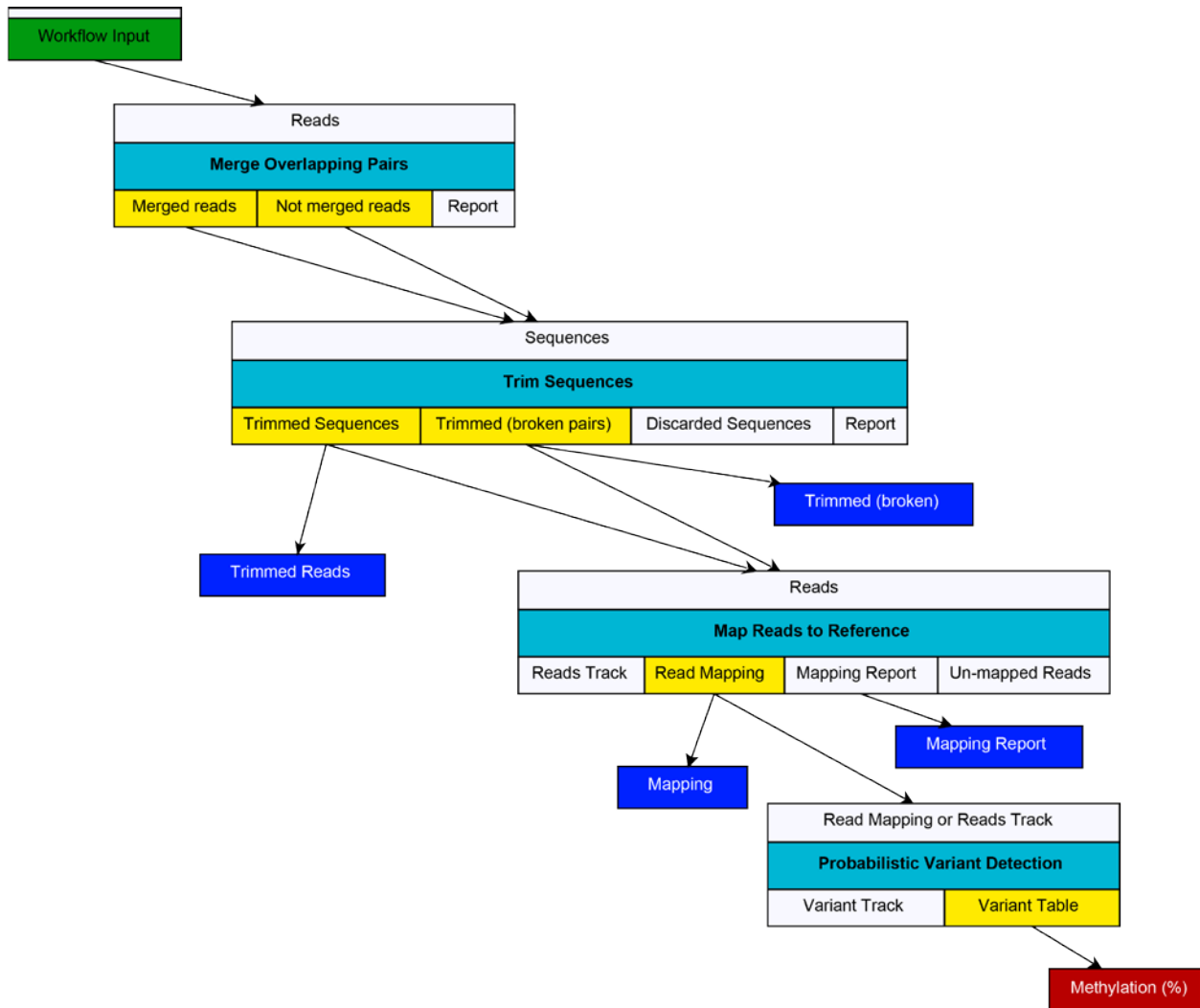
Supplemental Figure 1: Methylation quantitation workflow schematic. FastQ files are imported for workflow input. Reads are then merged to eliminate overlapping pairs. Sequences are then quality trimmed and mapped to a reference sequence. Variant detection is used to identify CpG sites and the percent cytosine methylation.
