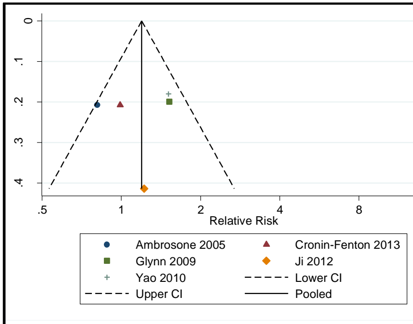
Figure B: Funnel plot showing little evidence of publication bias in studies investigating the association of any SOD2 polymorphisms with outcomes in breast cancer patients.
