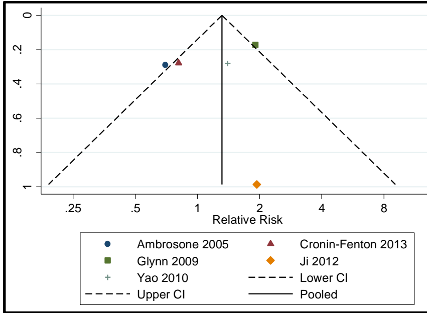
Figure B: Funnel plot showing little evidence of publication bias in studies investigating the association of any SOD2 polymorphisms with outcomes in breast cancer patients.
