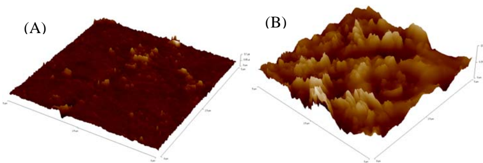
Figure S1. Example topography images of the original plastic surface (A) and the coated surface (B) based on AFM characterization.
