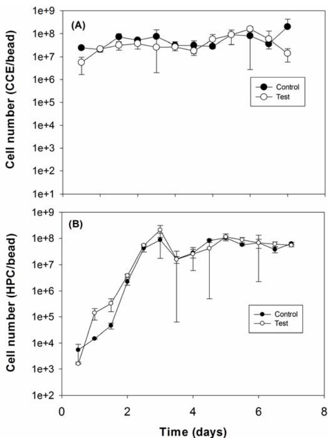
Figure S2. Biofilm biomass as indicated by the qPCR quantified calibrator cell equivalence (CCE/bead) (A) and heterotrophic plate count (HPC/bead) (B) during the third independent reactor startup.
