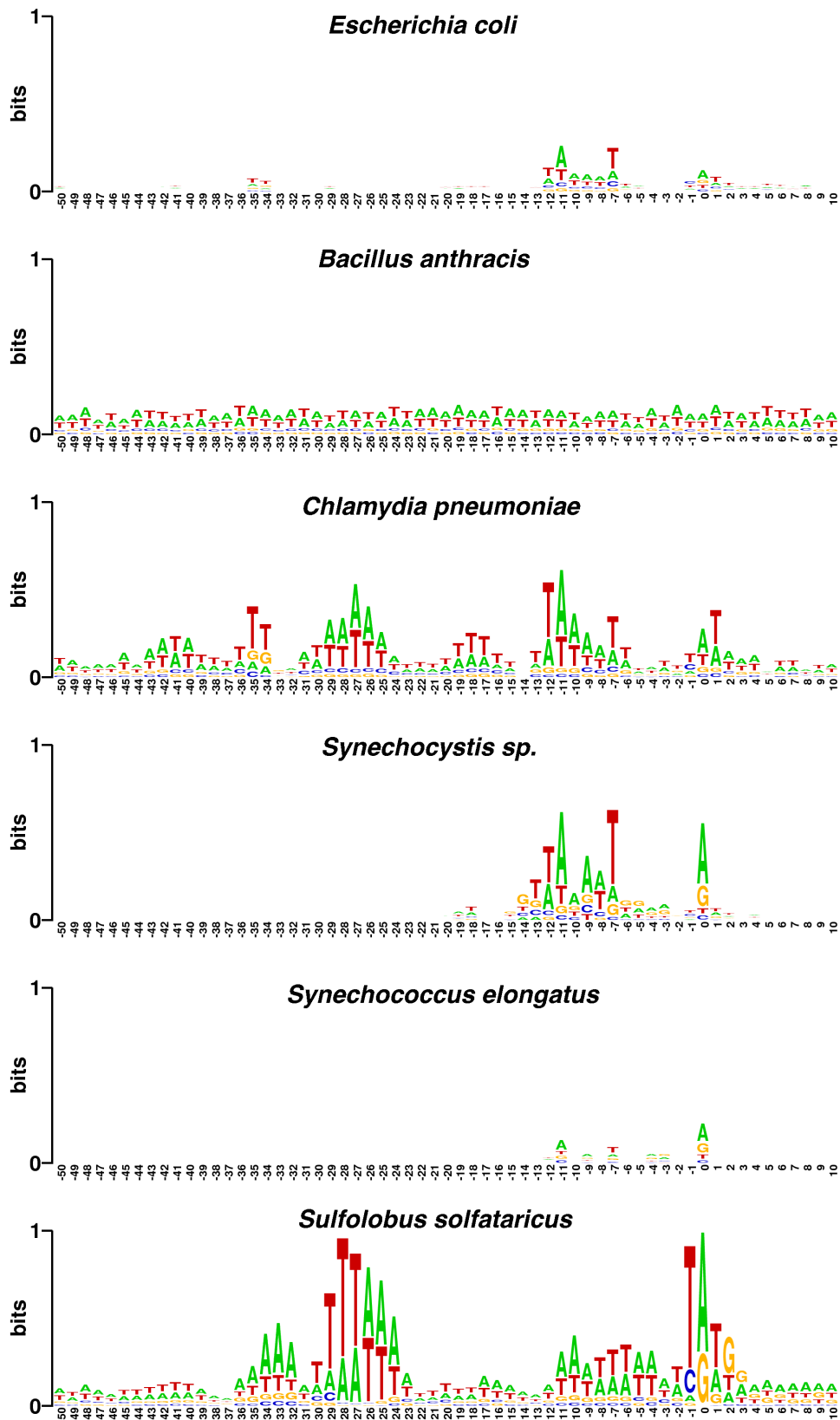
Supplemental figure S8: Motif logos generated with Weblogo of the promoter regions (50bp upstream to 10bp downstream of the TSS) for the six prokaryotes from different phyla.
