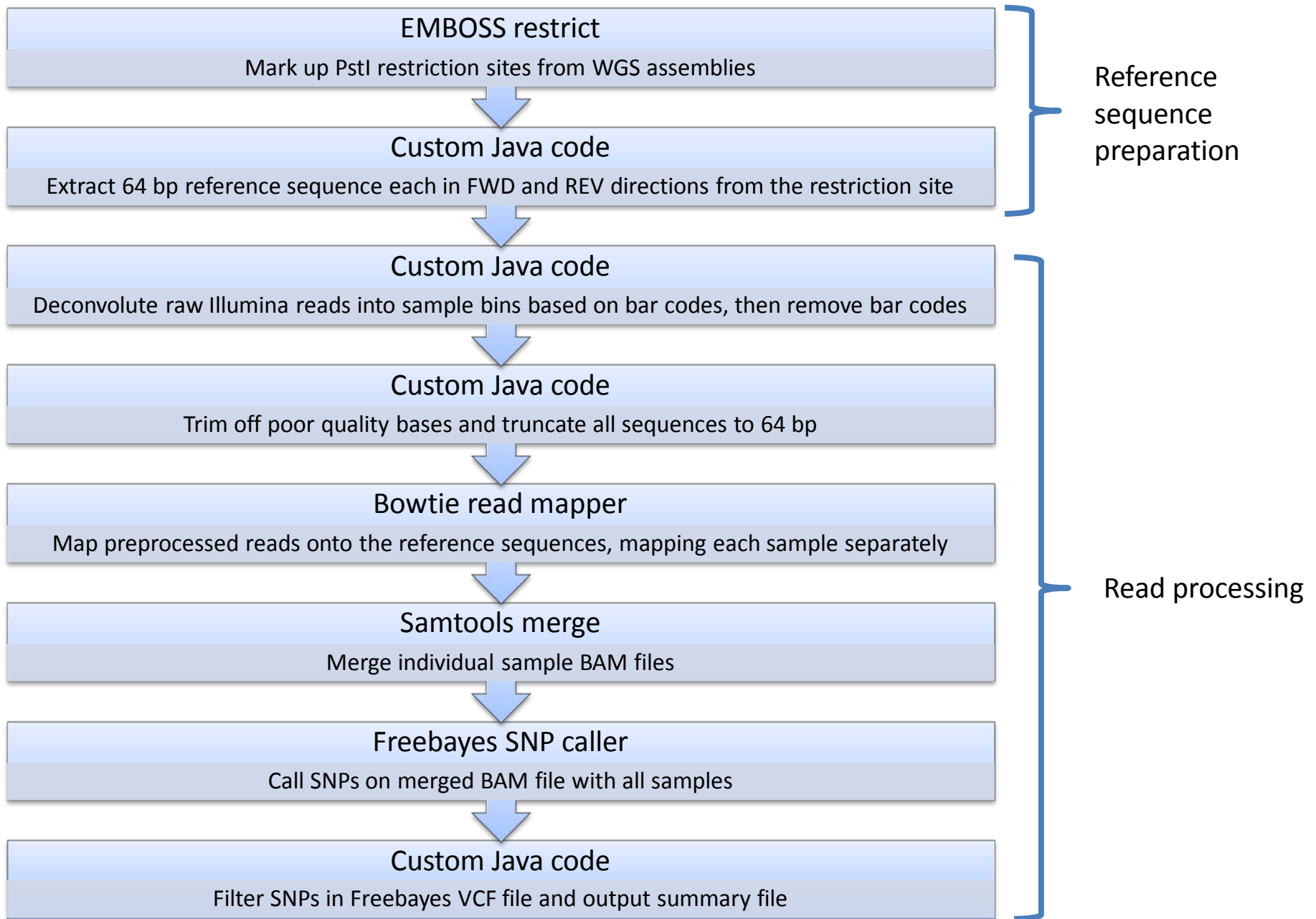
Supplementary Figure 1. Data processing workflow for the raw GBS Illumina reads.
