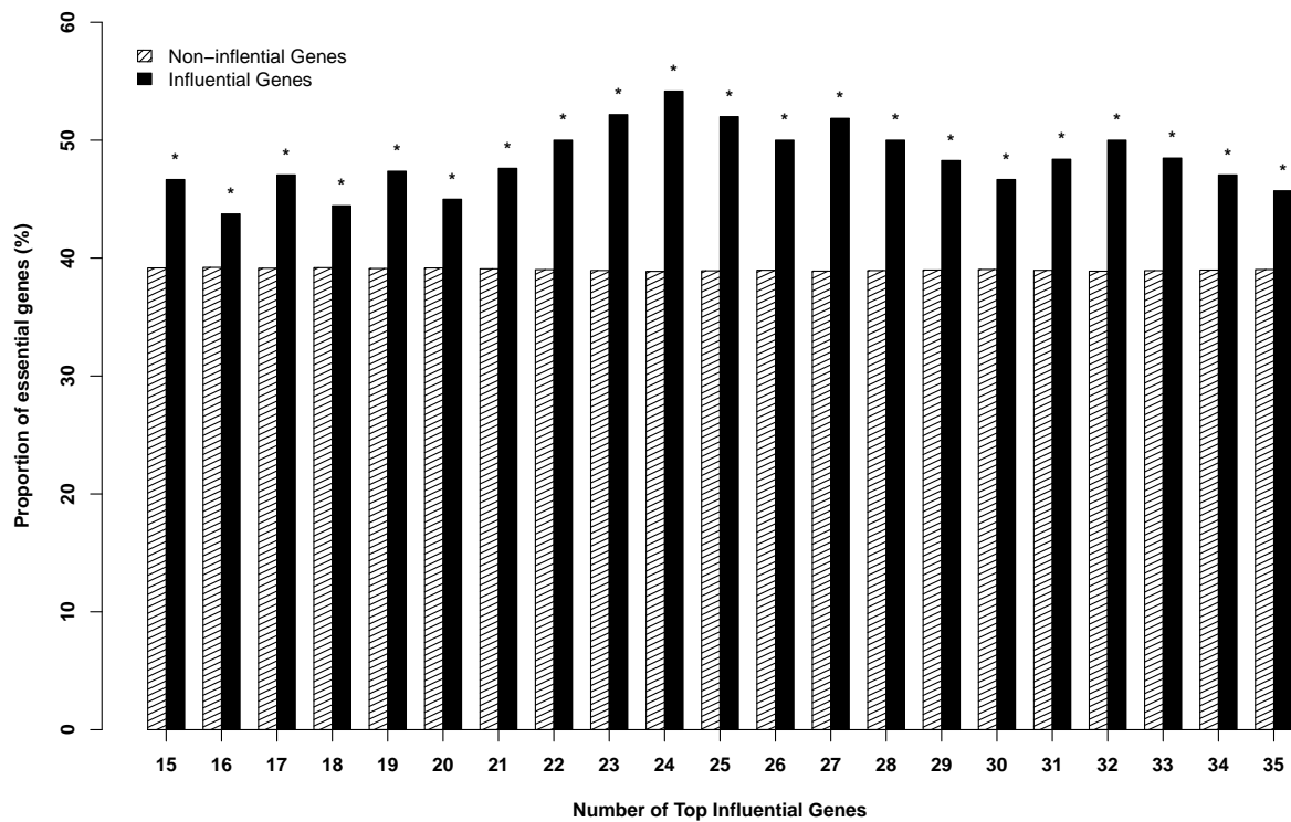
Supplemental Figure 1. Influential genes in a breast tumor coexpression network are enriched for essential genes at a range of thresholds. "*" indicates p \leq .001 calculated using the cumulative binomial distribution.
