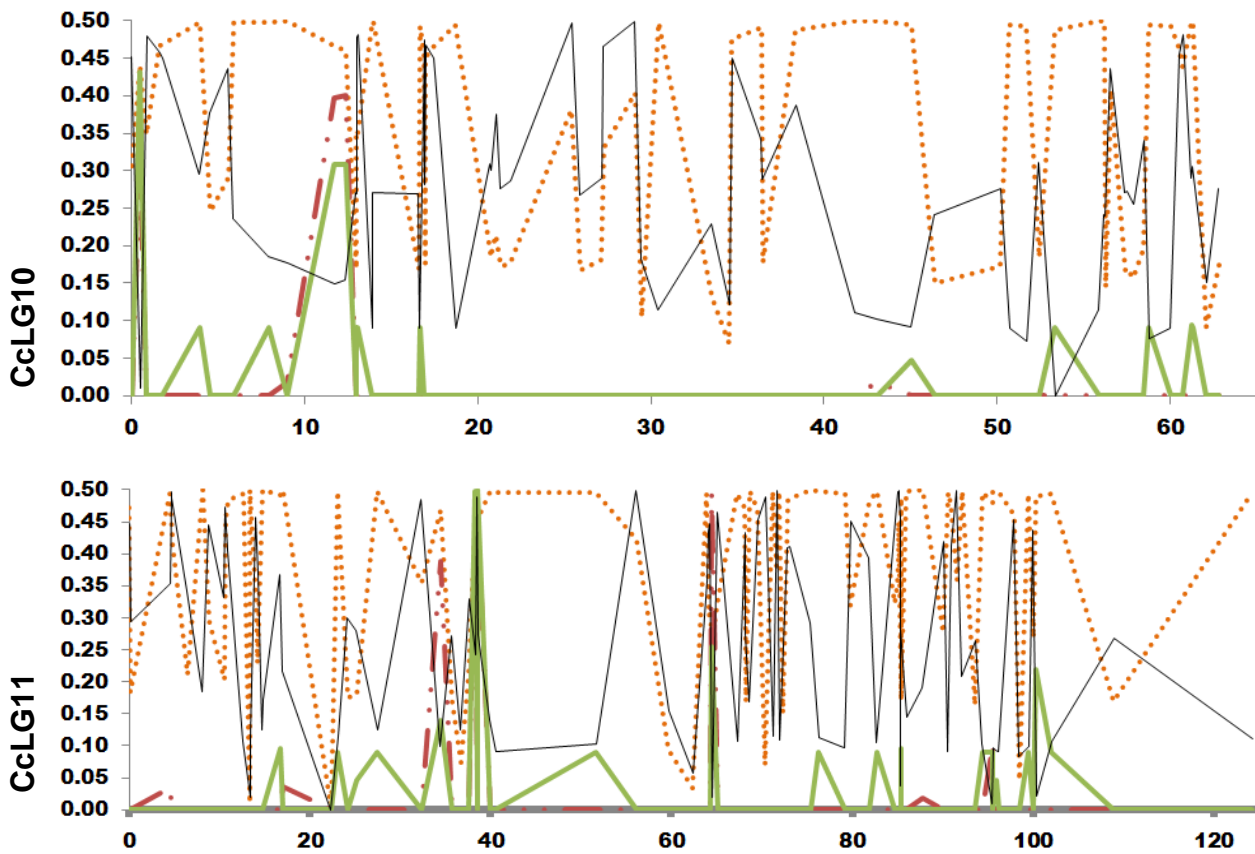
Figure S1: Estimated genome wide (CcLG01 to CcLG11) gene diversity using 875 mapped loci. “X” axis represents the length of each linkage group (CcLG) in cM and “Y” axis represents the value of gene diversity.
