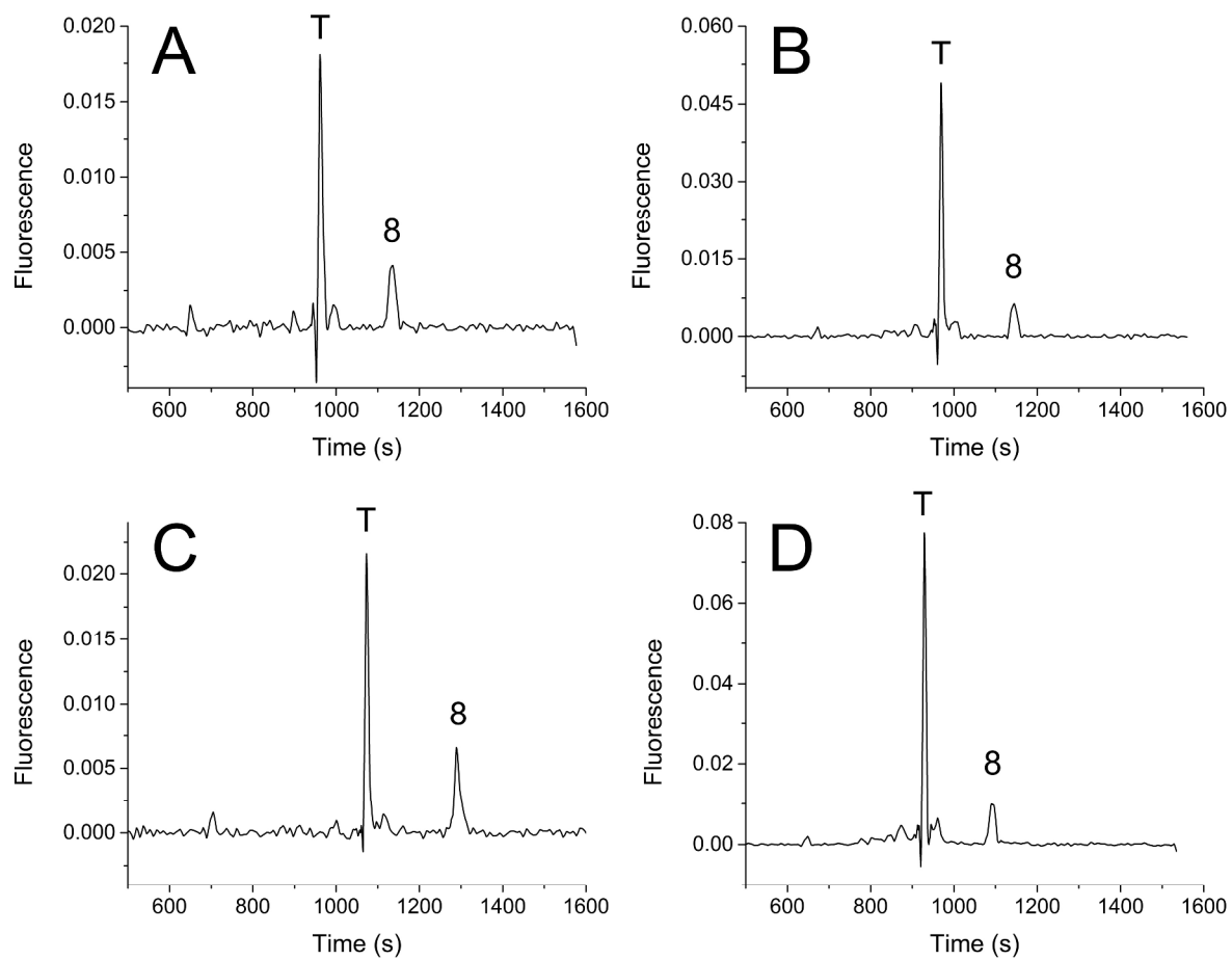
Figure S1. Fragmentation patterns for TS13 after incubation for (A) 3 h in A431 cell lysate or 5 min in a single (B) A431 cell, (C) BEAS-2B cell, (D) or primary hAEC. Peaks representing TS13 are labelled “T” while those representing the 8-residue fragment are labelled “8”.
