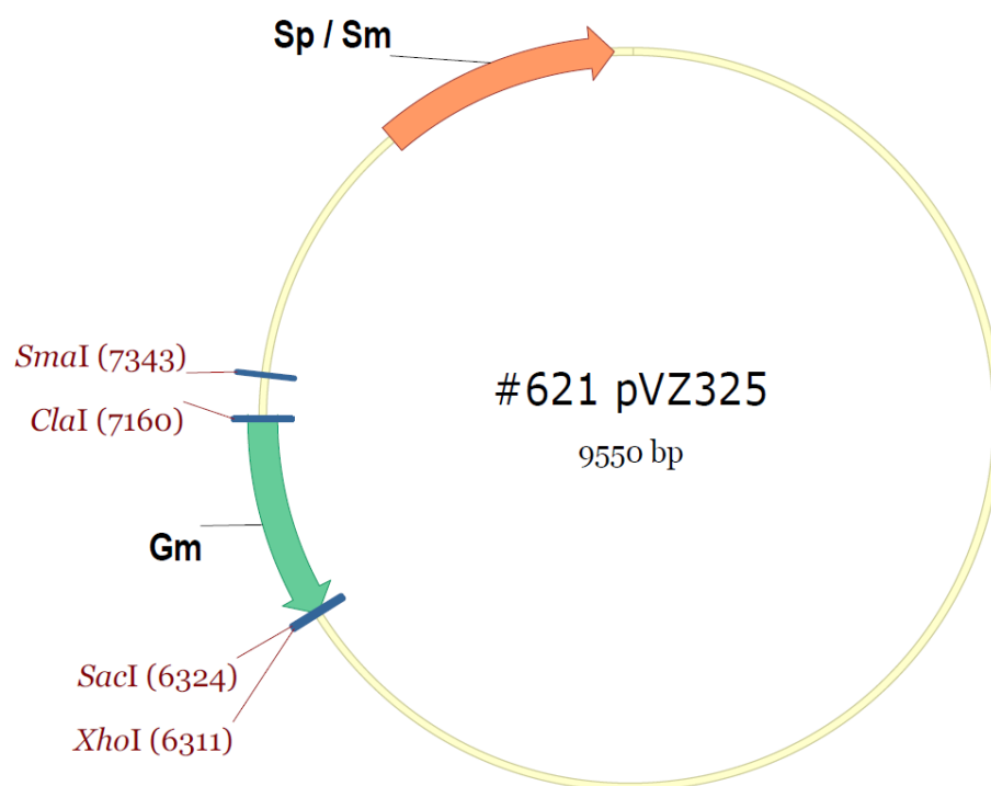
Figure 2. Non-ethanologenic empty-vector-control plasmid pVZ325 of isogenic control strain #621.
