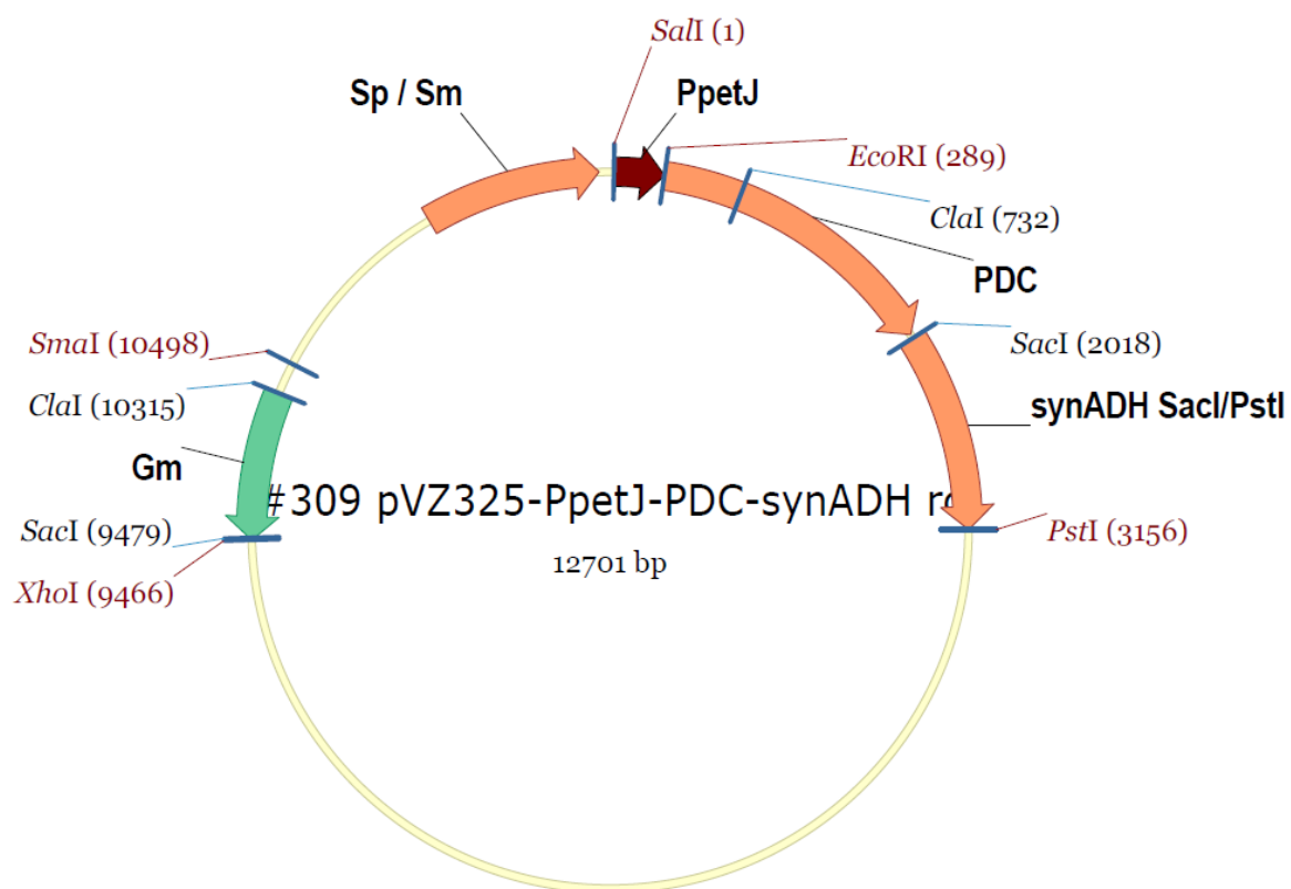
Figure 1. Ethanologenic plasmid pVZ325-PpetJ-PDC-synADH of producer strain #309.
