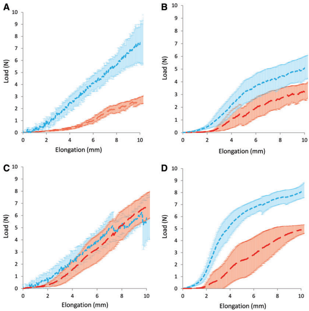
SUPPLEMENTARY FIG. S3. Average load–elongation curves of explanted meshes ( n=8 ) on (A, C) day 7 and (B, D) day 90 in mesh cross direction (A, B) and mesh machine direction (C, D). Dashed line indicates meshes implanted with eMSC, dotted line indicates meshes implanted without eMSC ( n=6 ). Error bars are 95% confidence intervals.
