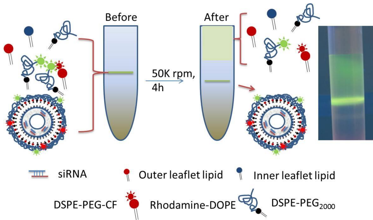
Figure S1. Schematic illustration of sucrose gradient centrifugation for purification.
