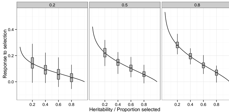
Figure 7: Response to selection 3 panels show simulations run at different heritability levels (.2, .5, .8), with varying proportions of selected individuals (.2, .4, .6, .8) (100 simulations, each). The dark curves show the response values predicted from the Breeder's Equation.
