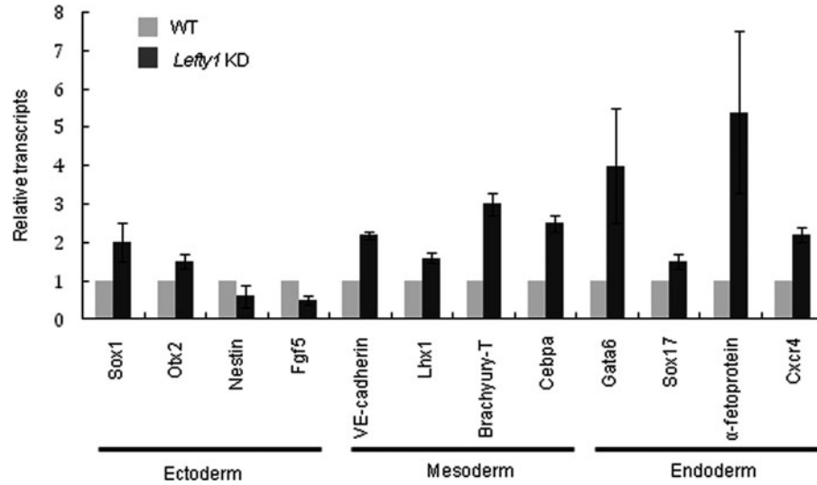
SUPPLEMENTARY FIG. S1. Lefty1 KD cells were spontaneously differentiated for 3 days and expression of the indicated genes was analyzed by real-time reverse transcriptase (RT)-PCR.
