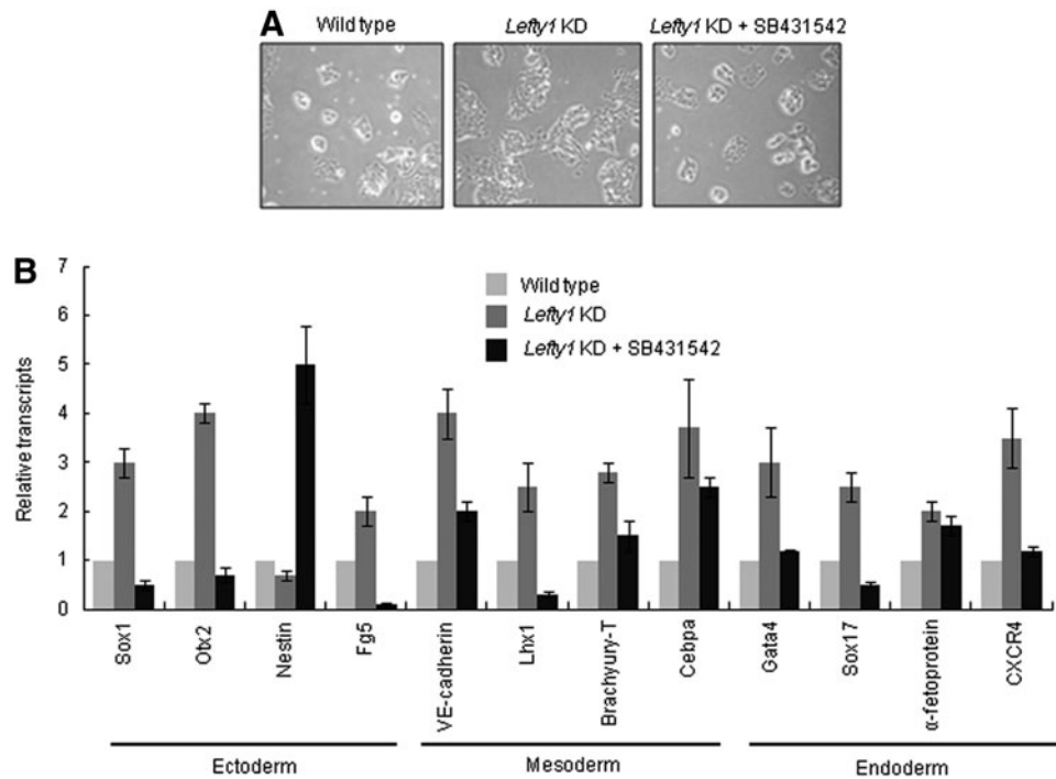
SUPPLEMENTARY FIG. S3. Lefty1 KD cells were differentiated for 3 days by removing LIF and adding RA in the presence or absence of SB431542 (20 \mu M). Cell morphology ( A ) and the expression of lineage markers ( B ) was analyzed by real-time RT-PCR. All values are expressed as the mean \pm SD of at least three independent experiments.
