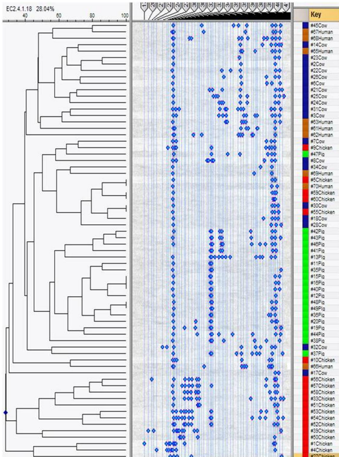
Supplementary Figure S1. Dendrogram of microbial profiles among 4 hosts analyzed by denaturing gradient gel electrophoresis (DGGE) analysis.
