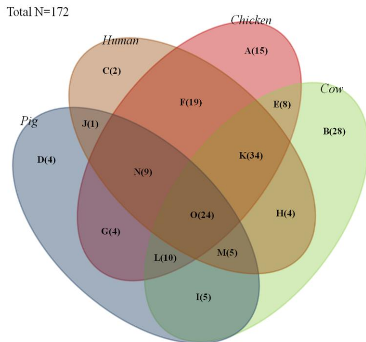
Supplementary Figure S3. Venn diagram comparing the genus level in (a) 16S rRNA gene, and OGBU level in (b) gBE gene.
