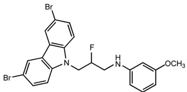
SUPPLEMENTARY FIG. 1. Chemical structure of P7C3-A20.
