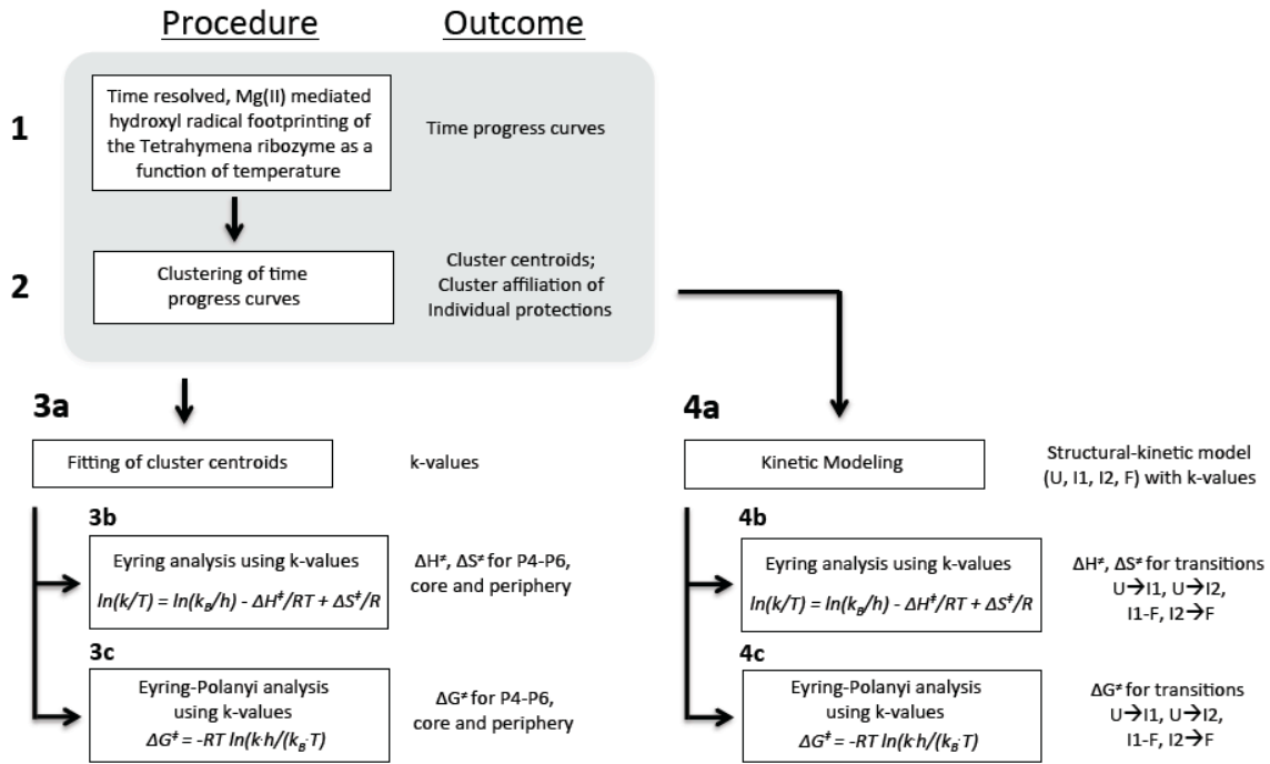
Figure S1. Roadmap for the study “Mapping the kinetic barriers of a large RNA molecule’s folding landscape”.
